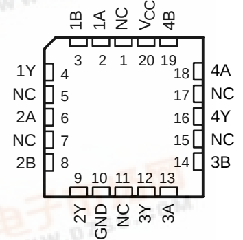
SN54AHCT86 . . . FK PACKAGE (TOP VIEW)
