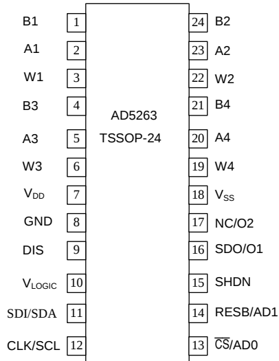
AD5263 PIN CONFIGURATION
