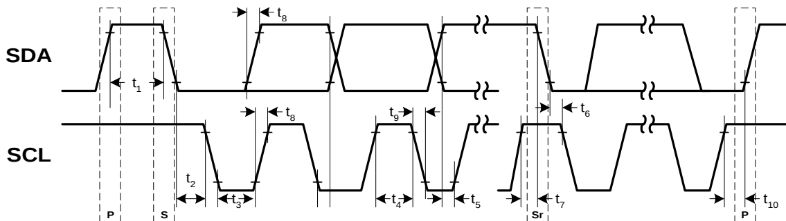
Figure 2. I 2 C Compatible Detail Timing Diagram
