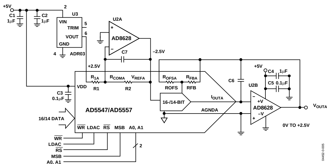
Figure 23. Unipolar 2-Quadrant Multiplying Mode, V_{OUT} = 0 to +V_{REF}
