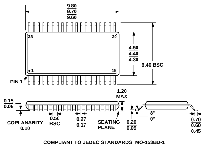
Figure 27. 38-Lead Thin Shrink Small Outline Package [TSSOP] (RU-38)
