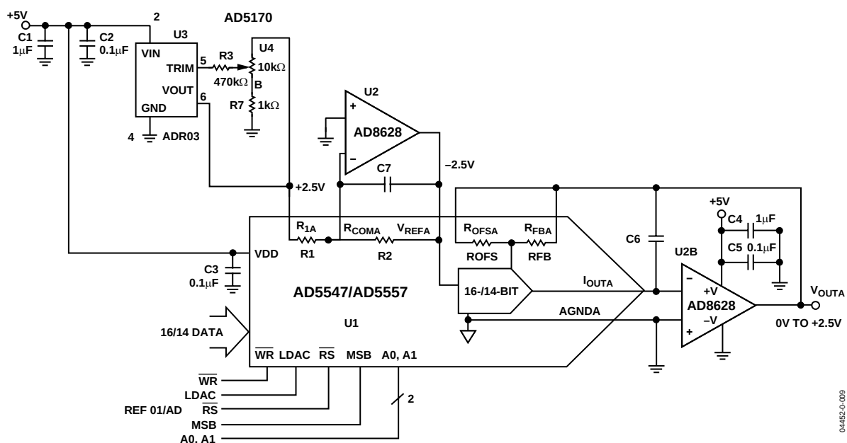
Figure 26. Full-Span Calibration
