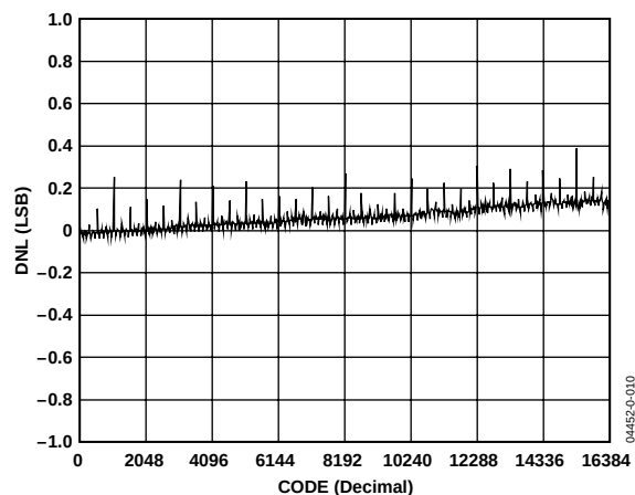
Figure 9. AD5557 Differential Nonlinearity Error
