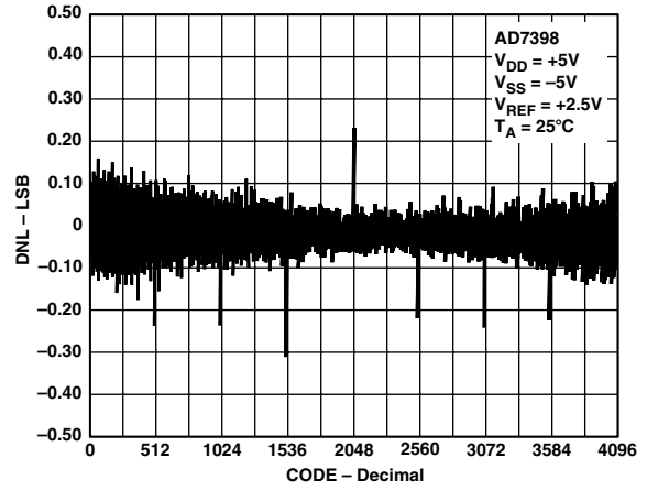
TPC 3. AD7398 DNL vs. Code ( T_A = 25^\circ C )
