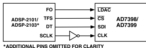
Figure 8. ADSP-2101/ADSP-2103 to AD7398/AD7399 Interface
