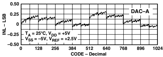
TPC 2. AD7399 INL vs. Code ( T_A = 25^\circ C )
