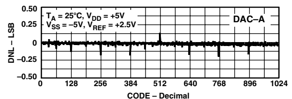
TPC 4. AD7399 DNL vs. Code ( T_A = 25^\circ C )
