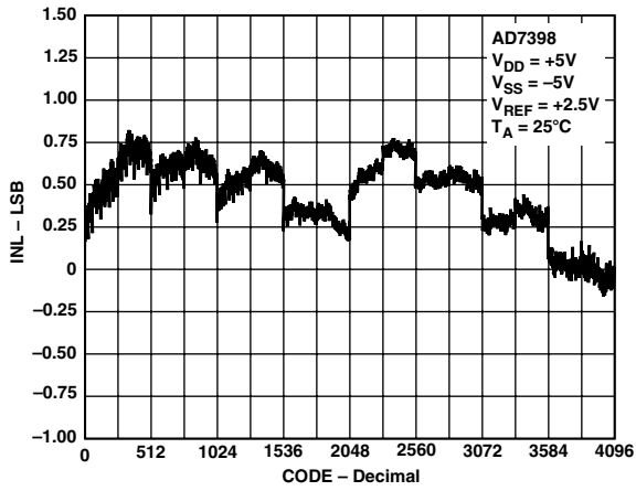
TPC 1. AD7398 INL vs. Code ( T_A = 25^\circ C )
