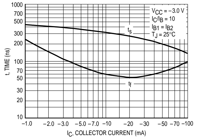
Figure 11. Turn-Off Time
