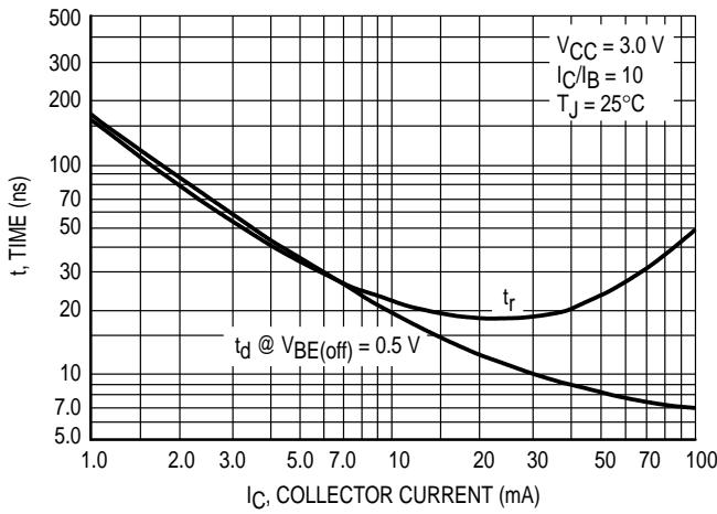
Figure 10. Turn-On Time
