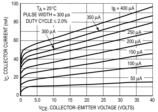
Figure 7. Collector Characteristics
