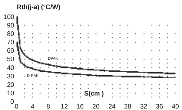
Fig. 10: DPAK and D 2 PAK Thermal resistance junction to ambient versus copper surface under tab (printed circuit board FR4, copper thickness: 35 \mu m).
