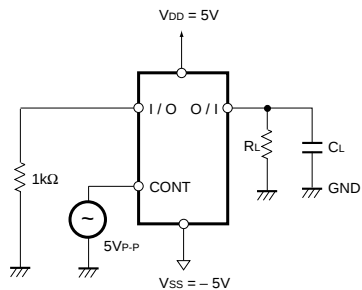
Fig. 2 (f) Control IN→OUT crosstalk
