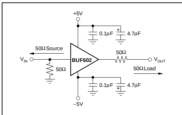
Figure 29. DC-Coupled, Bipolar Supply, Specification and Test Circuit
