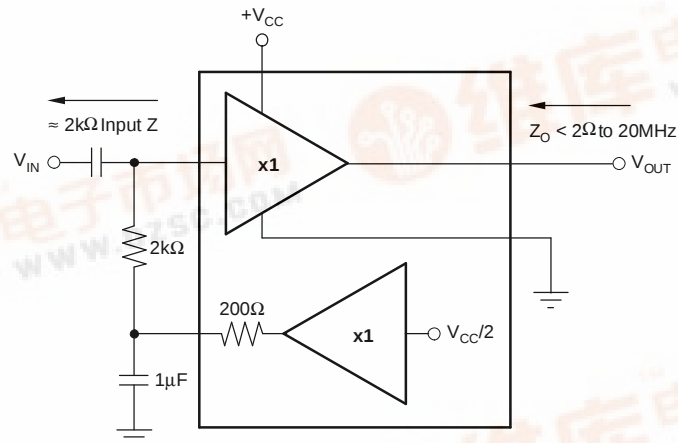
Self-Referenced, AC-Coupled, Single-Supply Buffer
