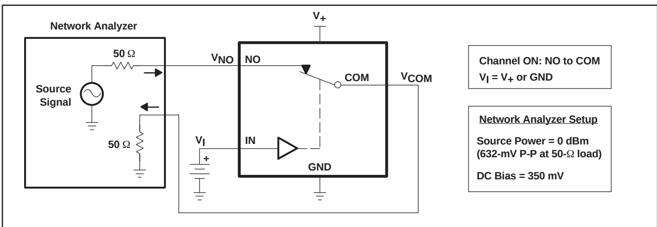
Figure 18. Bandwidth (BW)
