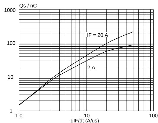
Fig.8. Maximum Q_s at T_j = 25^\circ\text{C} ; per diode.
