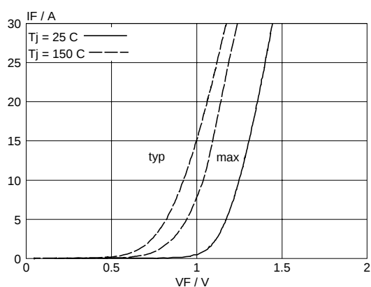
Fig.7. Typical and maximum forward characteristic
