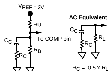
FIGURE 9. COMPENSATION CIRCUIT
