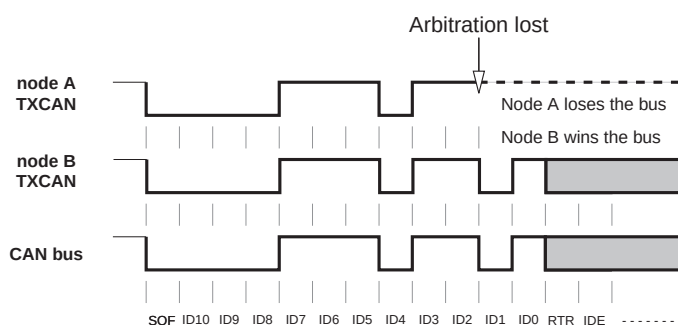
Figure 46. Bus Arbitration
