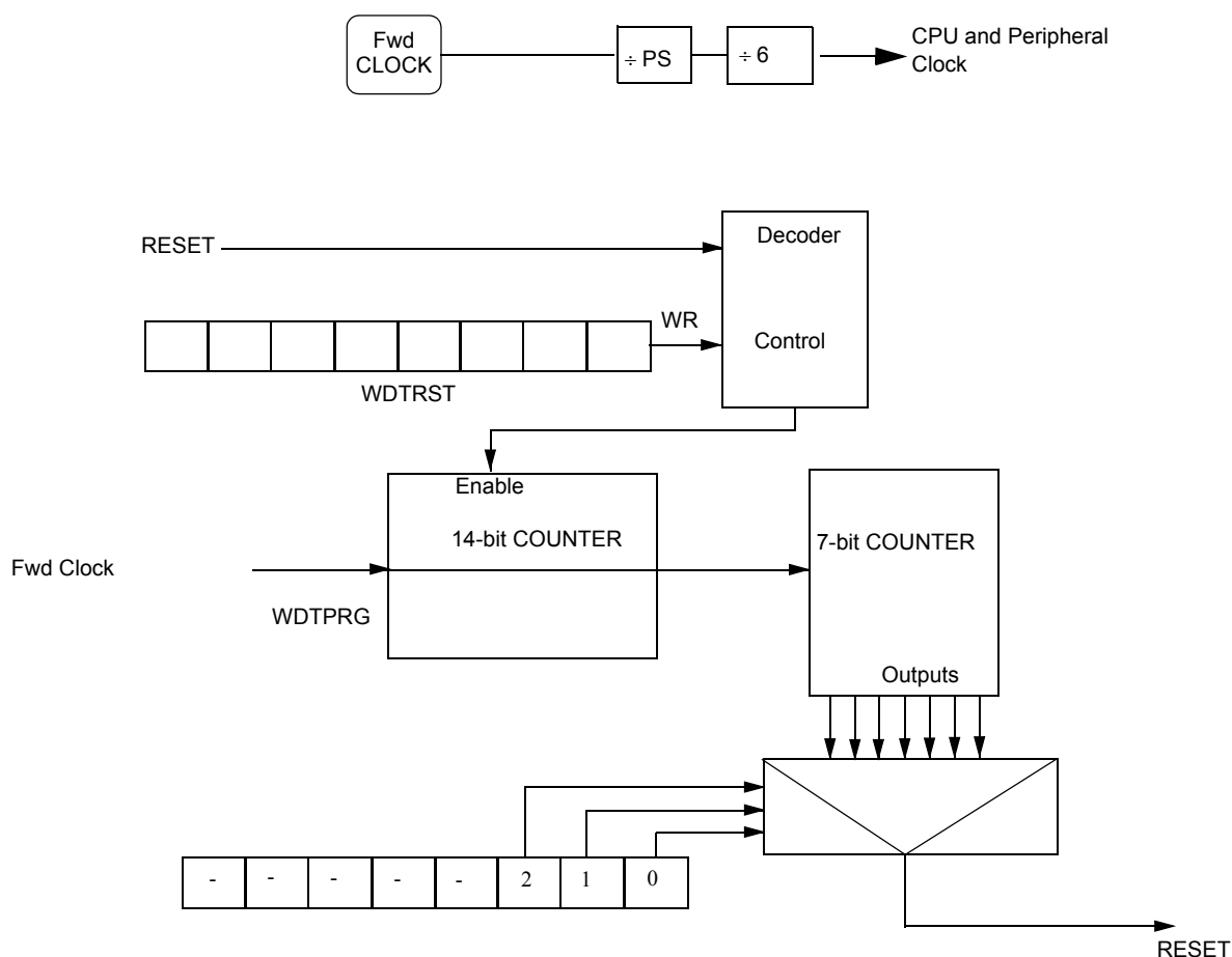
Figure 42. Watchdog Timer
