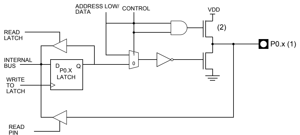
Figure 2. Port 0 Structure
