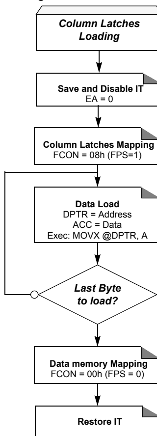
Figure 25. Column Latches Loading Procedure
