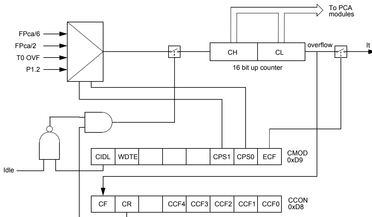
Figure 67. PCA Timer/Counter
