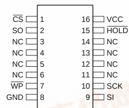
16-Pin SOIC
