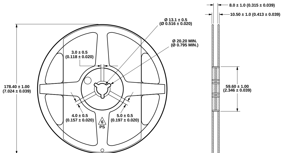
Figure 20. Reel dimensions.
