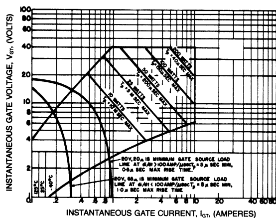
GATE CHARACTERISTICS
