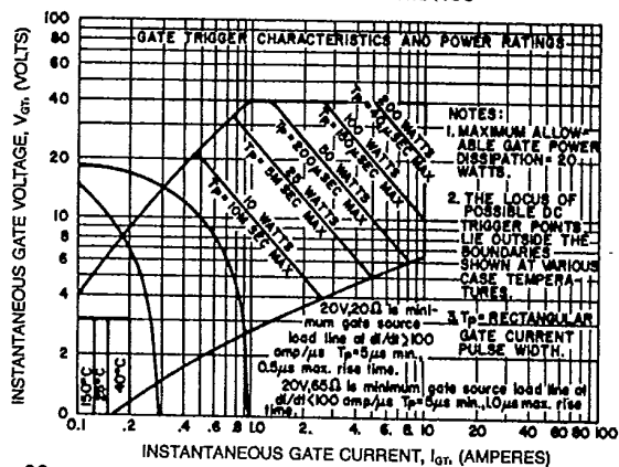
GATE CHARACTERISTICS
