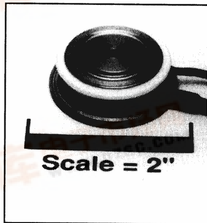
C380__X555 Phase Control SCR 300 Amperes Average, 1300 Volts
