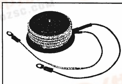
C390__X500 Phase Control SCR 620 Amperes/100-600 Volts
