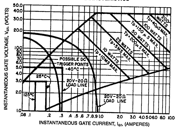
GATE CHARACTERISTICS
