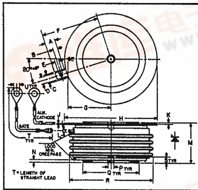
C441 Outline Drawing
