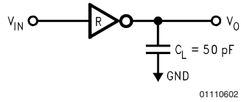
FIGURE 1. Receiver Load Circuit
