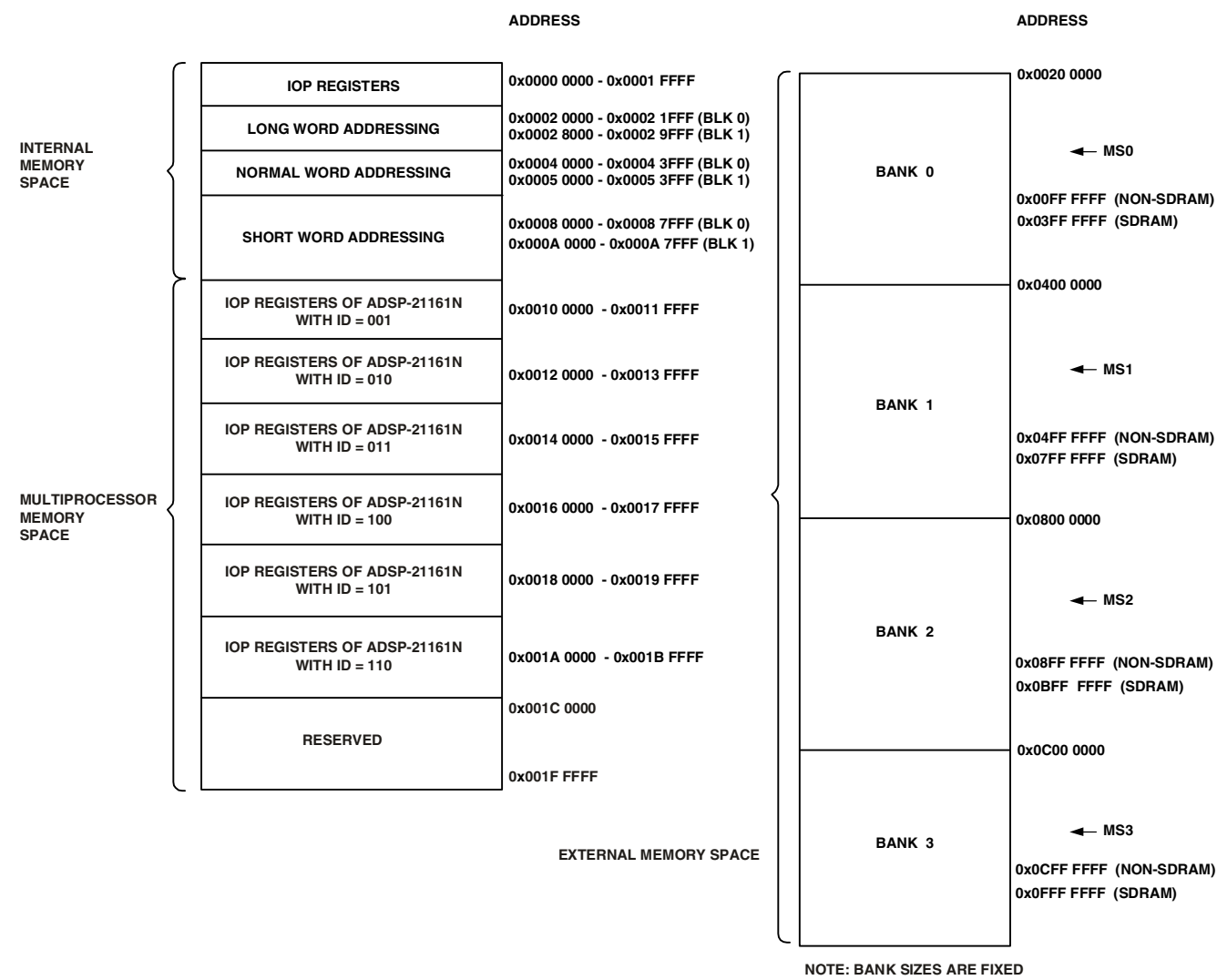
Figure 2. Memory Map
