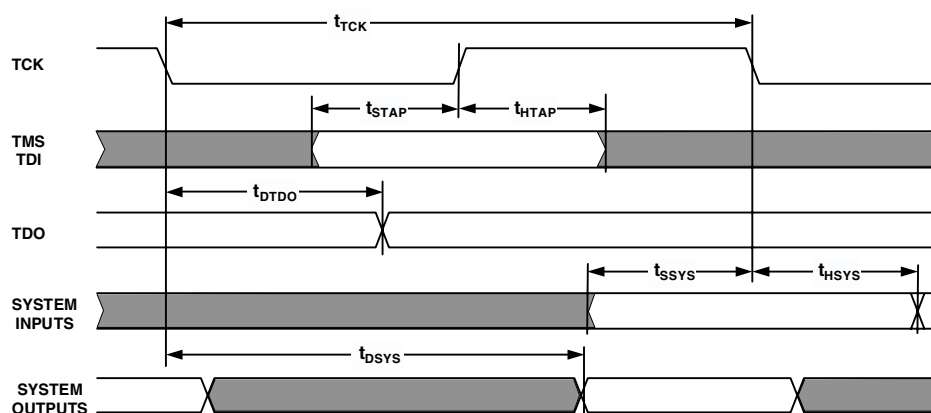
Figure 36. JTAG Test Access Port and Emulation
