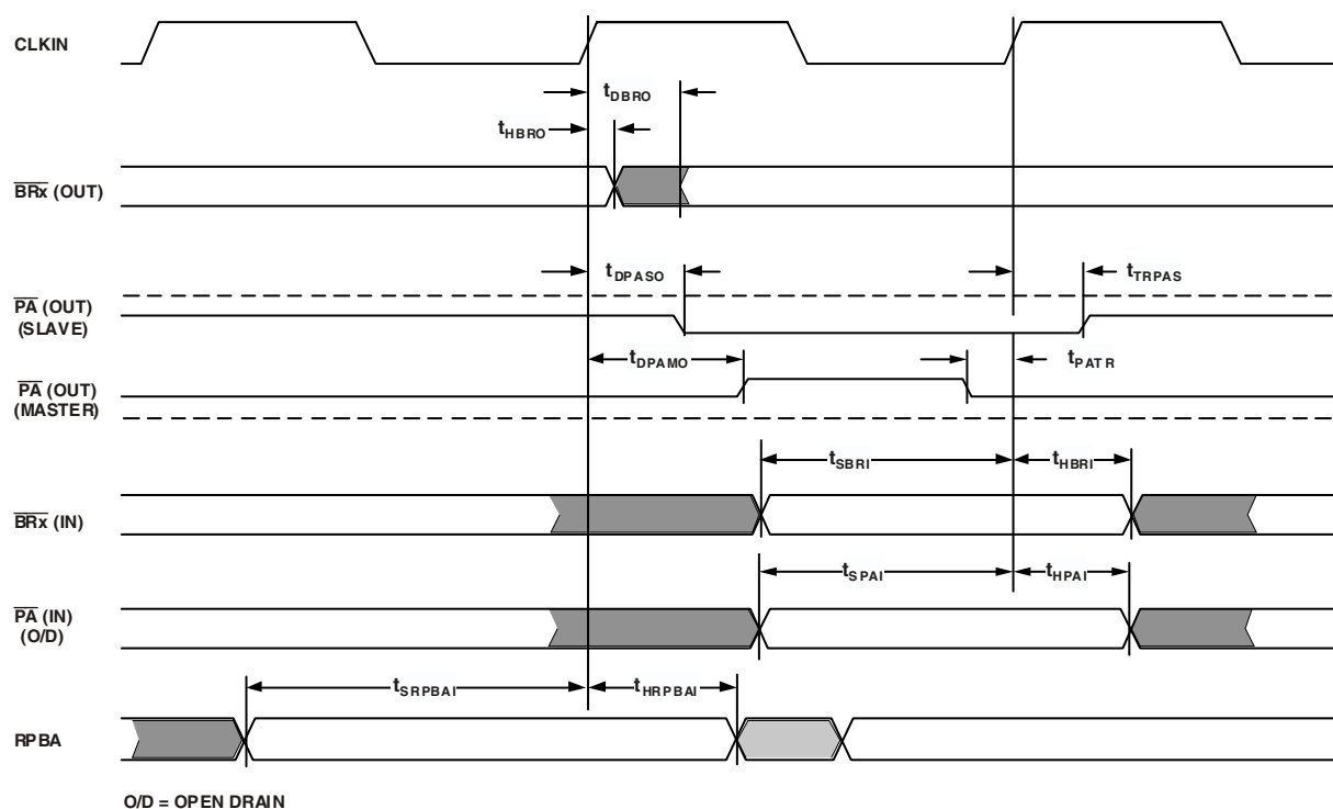
Figure 25. Multiprocessor Bus Request
