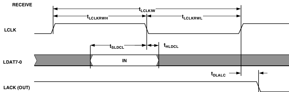
Figure 30. Link Ports—Receive
