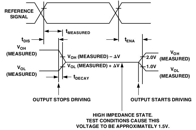
Figure 38. Output Enable/Disable
