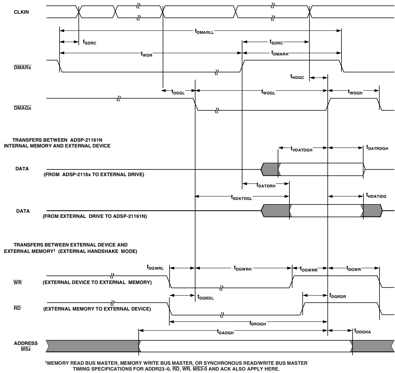
Figure 28. DMA Handshake
