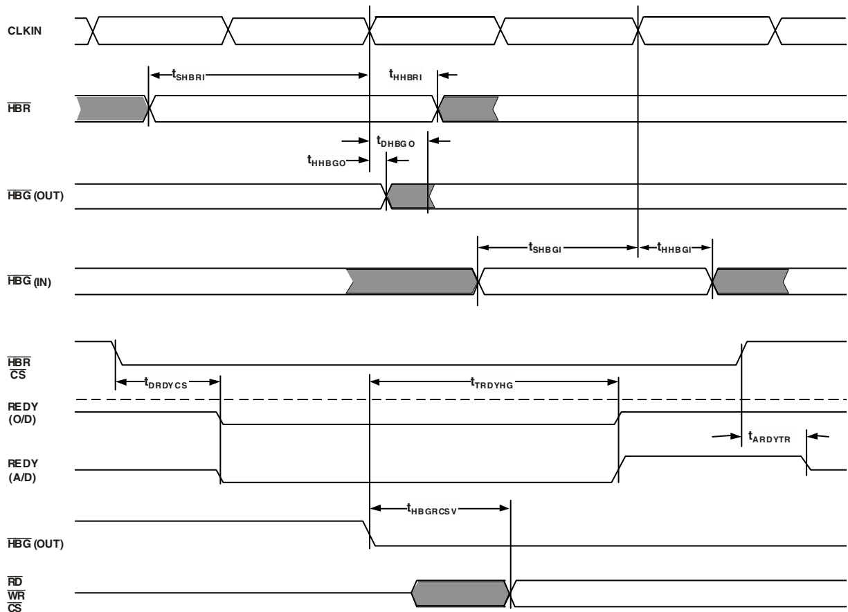
Figure 24. Host Bus Request
