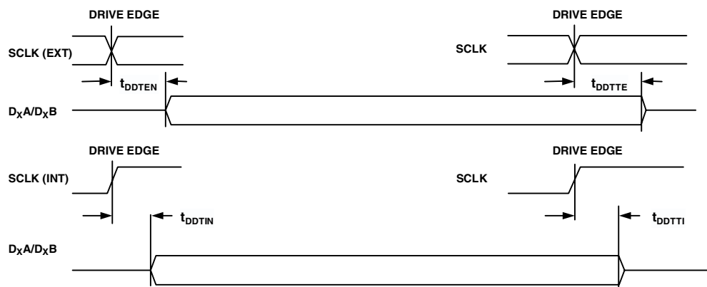
Figure 32. Serial Ports
