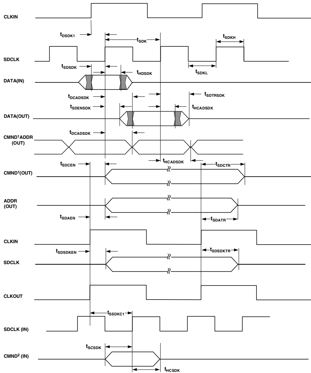
Figure 29. SDRAM Interface
