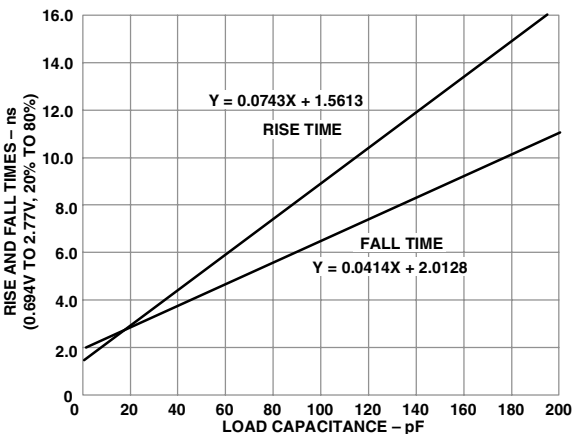
Figure 42. Typical Output Rise/Fall Time (20% - 80%, V_{DDEXT} = \text{Max} )
