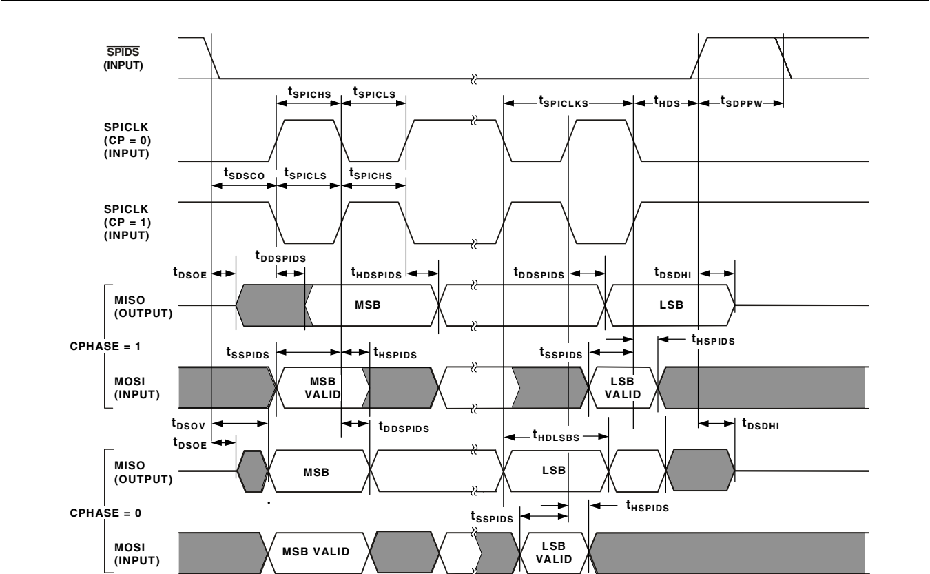
Figure 35. SPI Interface Protocol – Slave Switching and Timing
