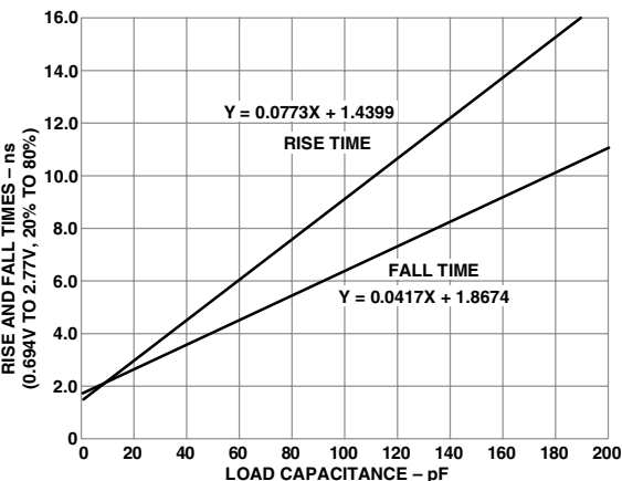
Figure 43. Typical Output Rise/Fall Time (20% - 80%, V_{DDEXT} = \text{Min} )
