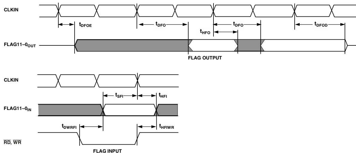
Figure 19. Flags
