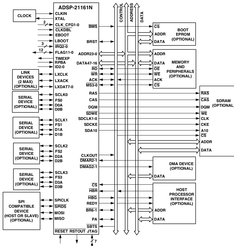
Figure 1. System Diagram
