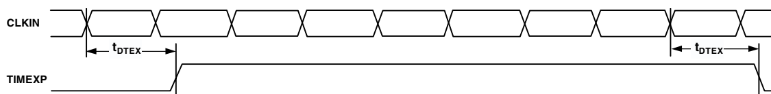
Figure 18. Timer
