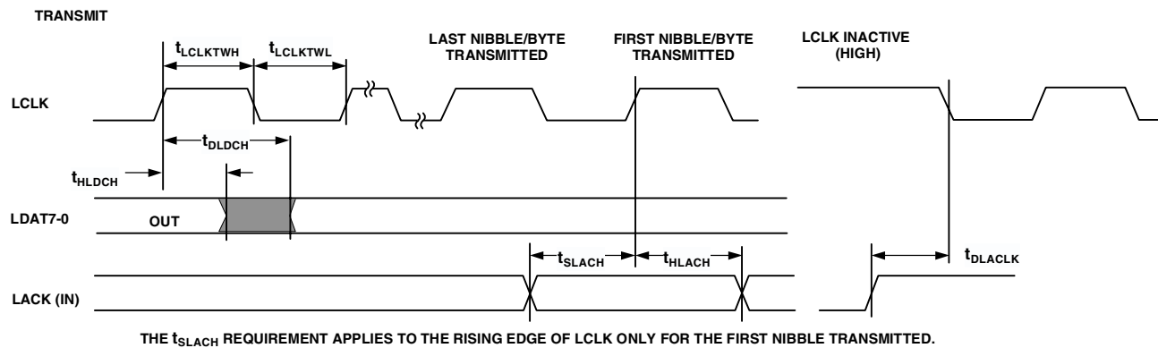
Figure 31. Link Ports—Transmit
