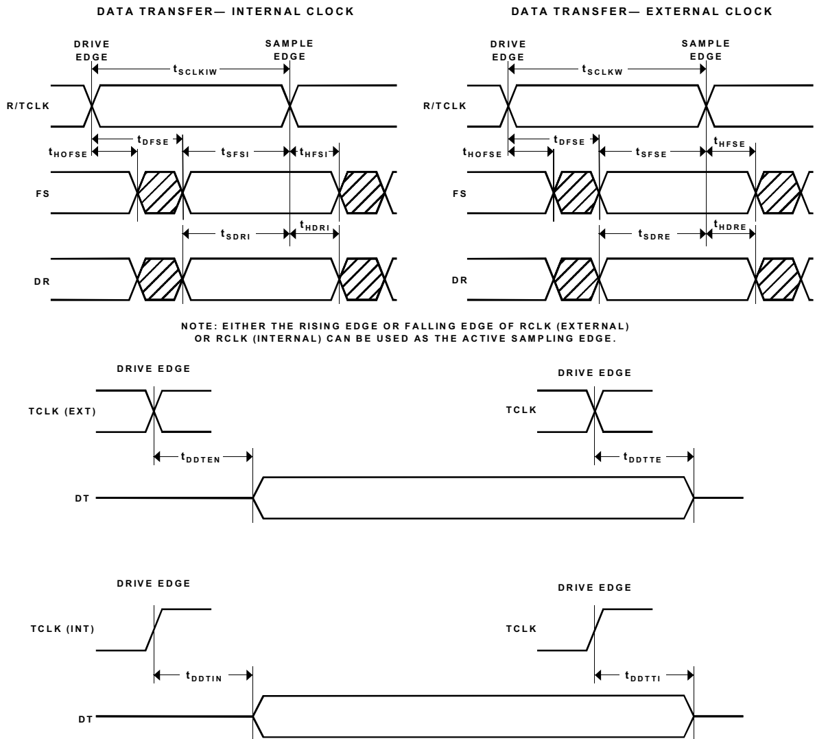
Figure 21. Serial Port (SPORT) Clocks and Data
