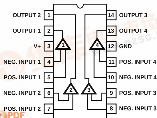
CA139A (SOIC) CA139, CA339, LM3302 (PDIP, SOIC) CA239, LM2901, LM339 (PDIP) TOP VIEW
