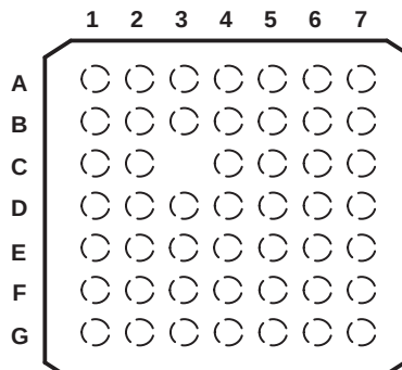
GQC PACKAGE (TOP VIEW)
