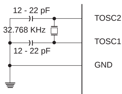
Figure 74. Timer/Counter2 Crystal Oscillator Connections
