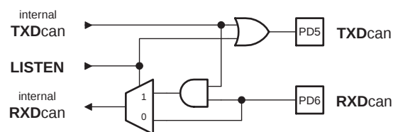
Figure 116. Listening Mode
