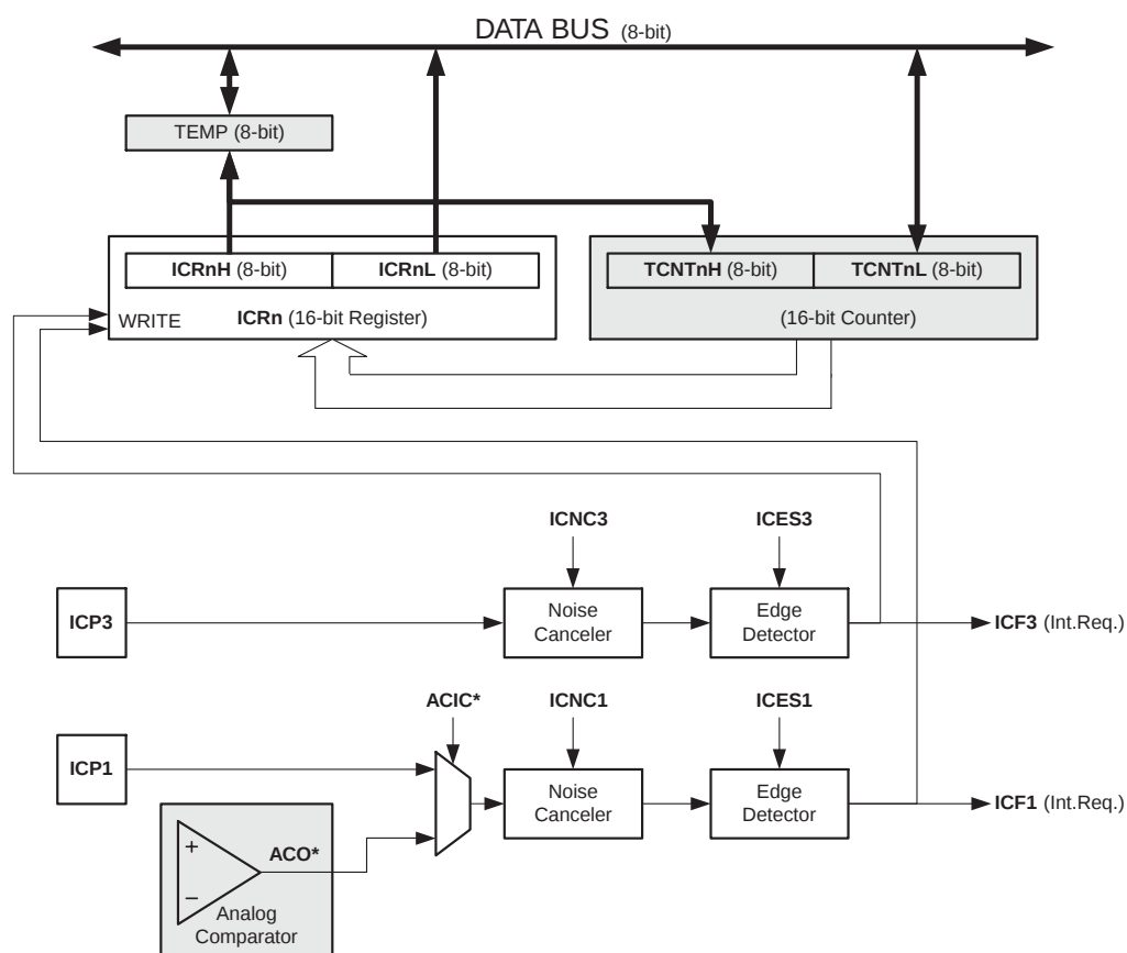
Figure 50. Input Capture Unit Block Diagram
