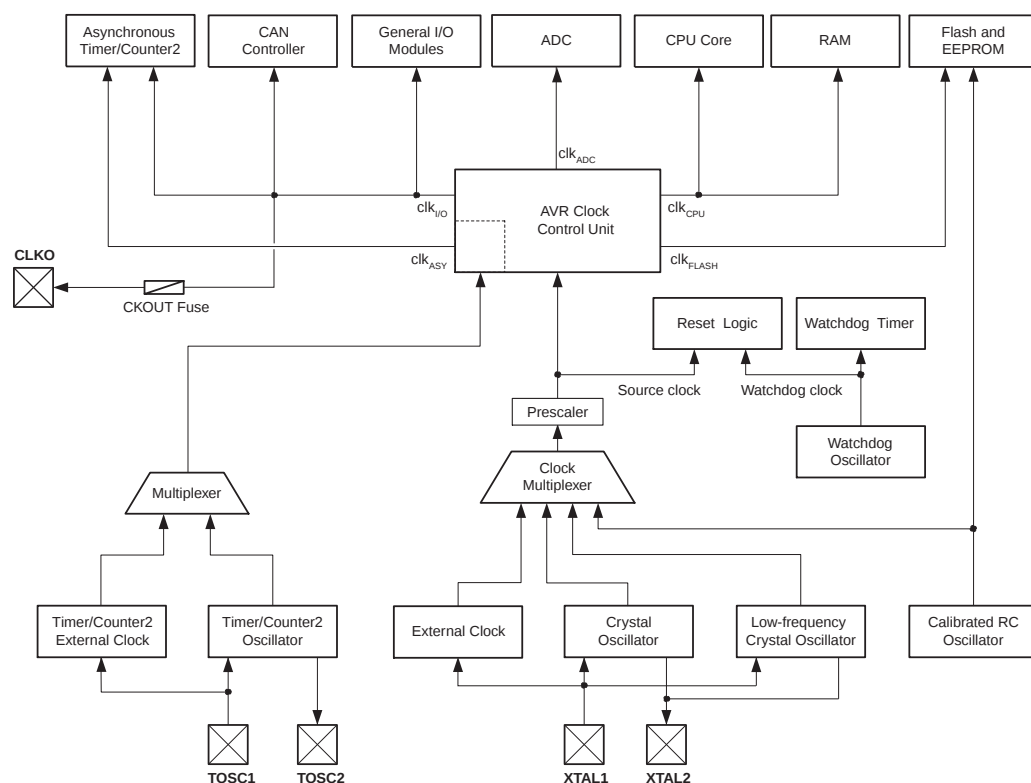
Figure 19. Clock Distribution
