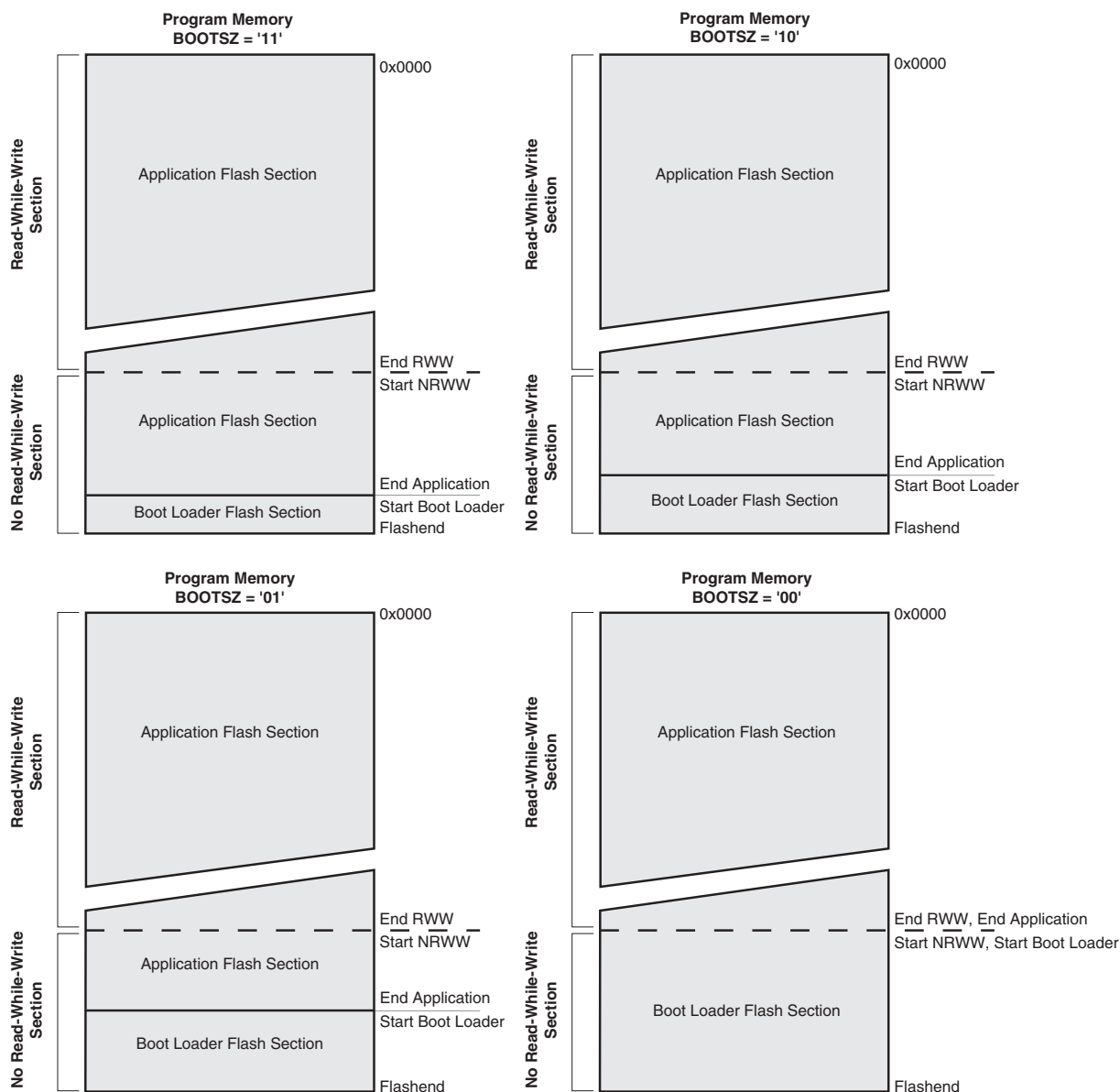
Figure 154. Memory Sections
