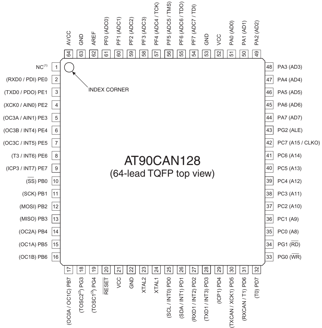
Figure 2. Pinout AT90CAN128- TQFP
