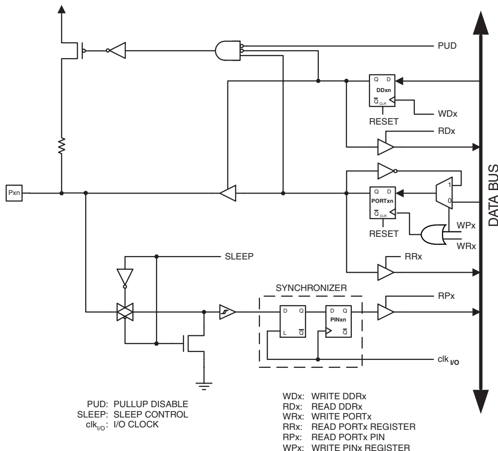
Figure 31. General Digital I/O (1)
