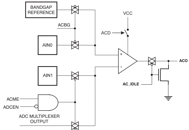
Figure 150. Analog Comparator
