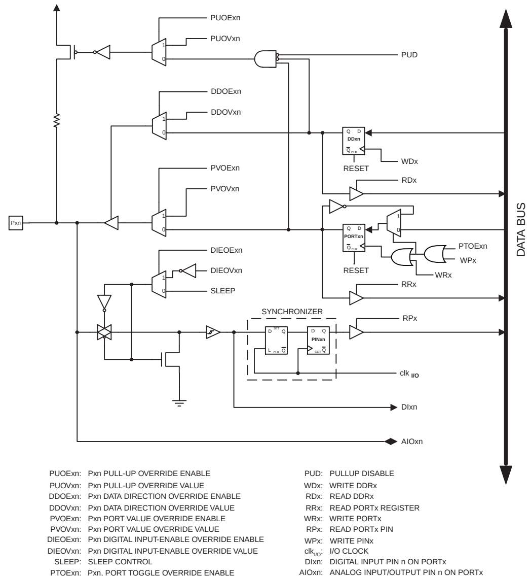
Figure 34. Alternate Port Functions (1)
