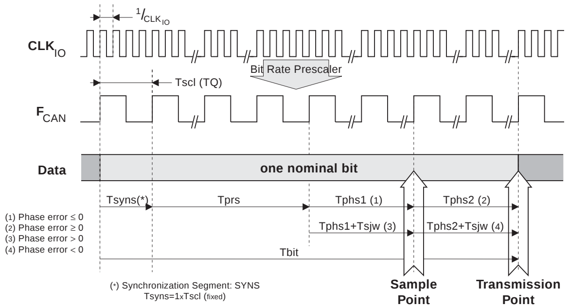
Figure 118. General Structure of a Bit Period
