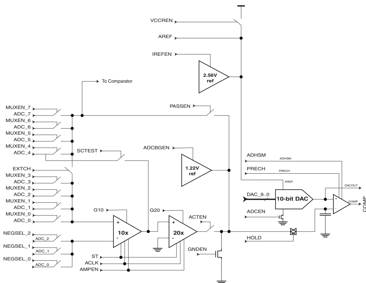
Figure 152. Analog to Digital Converter
