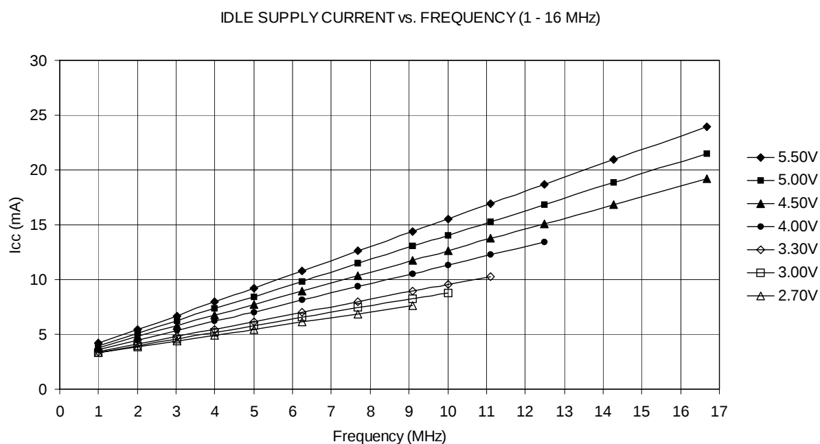
Figure 186. Idle Supply Current vs. Frequency (1 - 16 MHz)
