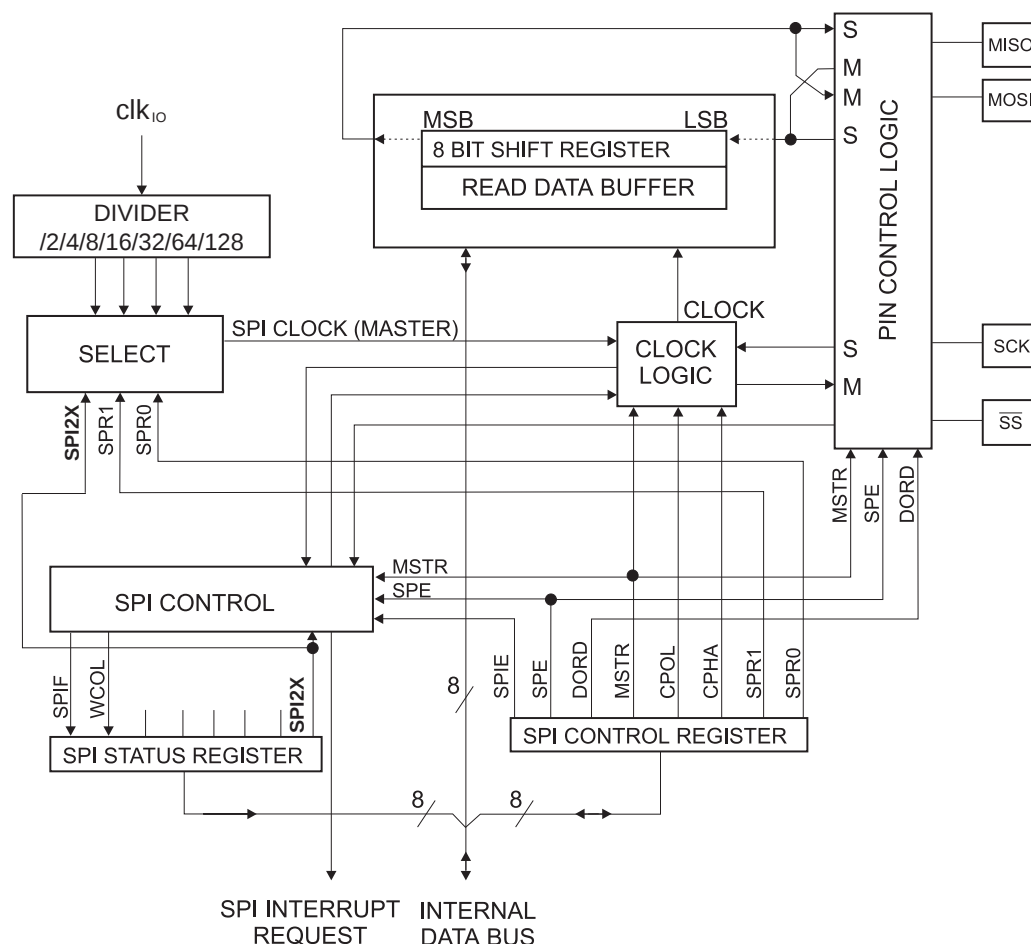
Figure 79. SPI Block Diagram (1)
