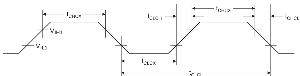
Figure 169. External Clock Drive Waveforms
