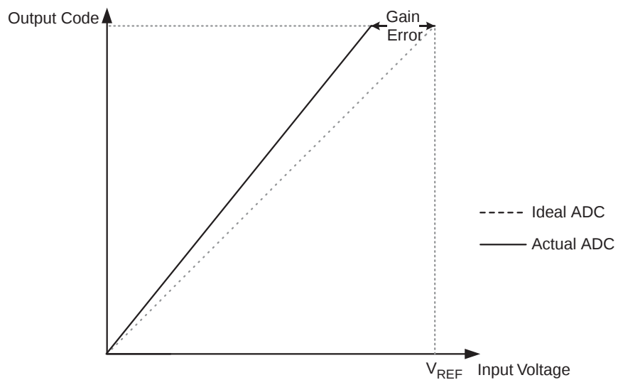
Figure 137. Gain Error
