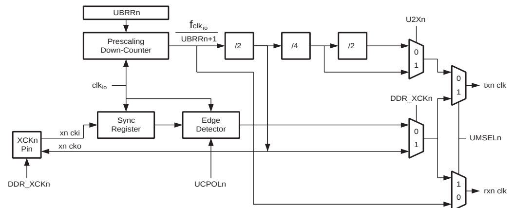
Figure 84. USARTn Clock Generation Logic, Block Diagram
