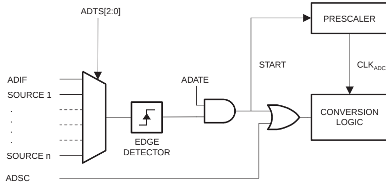
Figure 128. ADC Auto Trigger Logic
