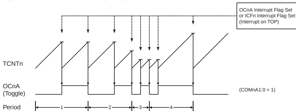
Figure 53. CTC Mode, Timing Diagram
