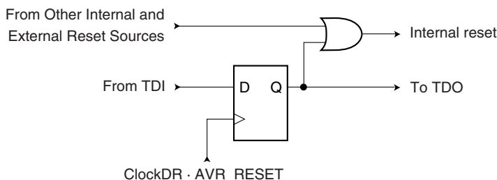
Figure 144. Reset Register
