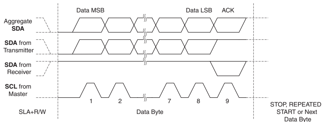
Figure 94. Data Packet Format
