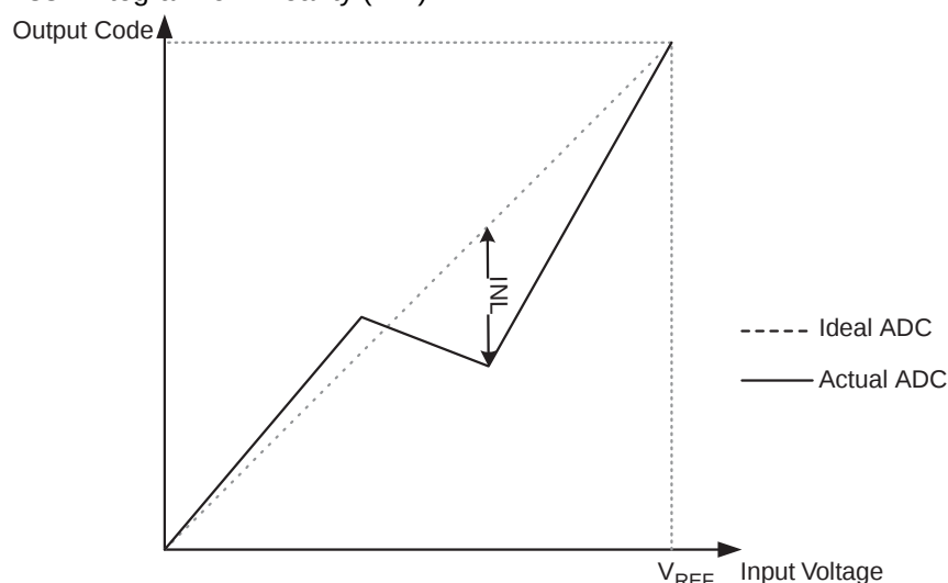
Figure 138. Integral Non-linearity (INL)
