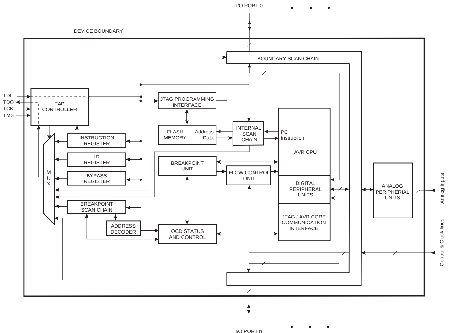
Figure 141. Block Diagram
