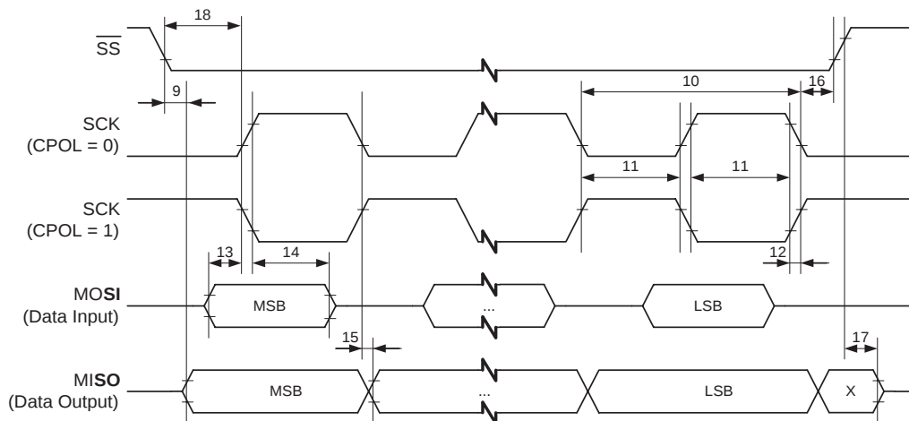
Figure 172. SPI Interface Timing Requirements (Slave Mode)
