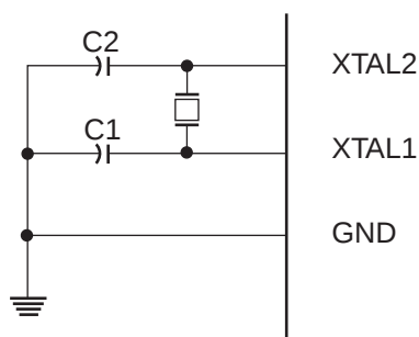
Figure 20. Crystal Oscillator Connections
