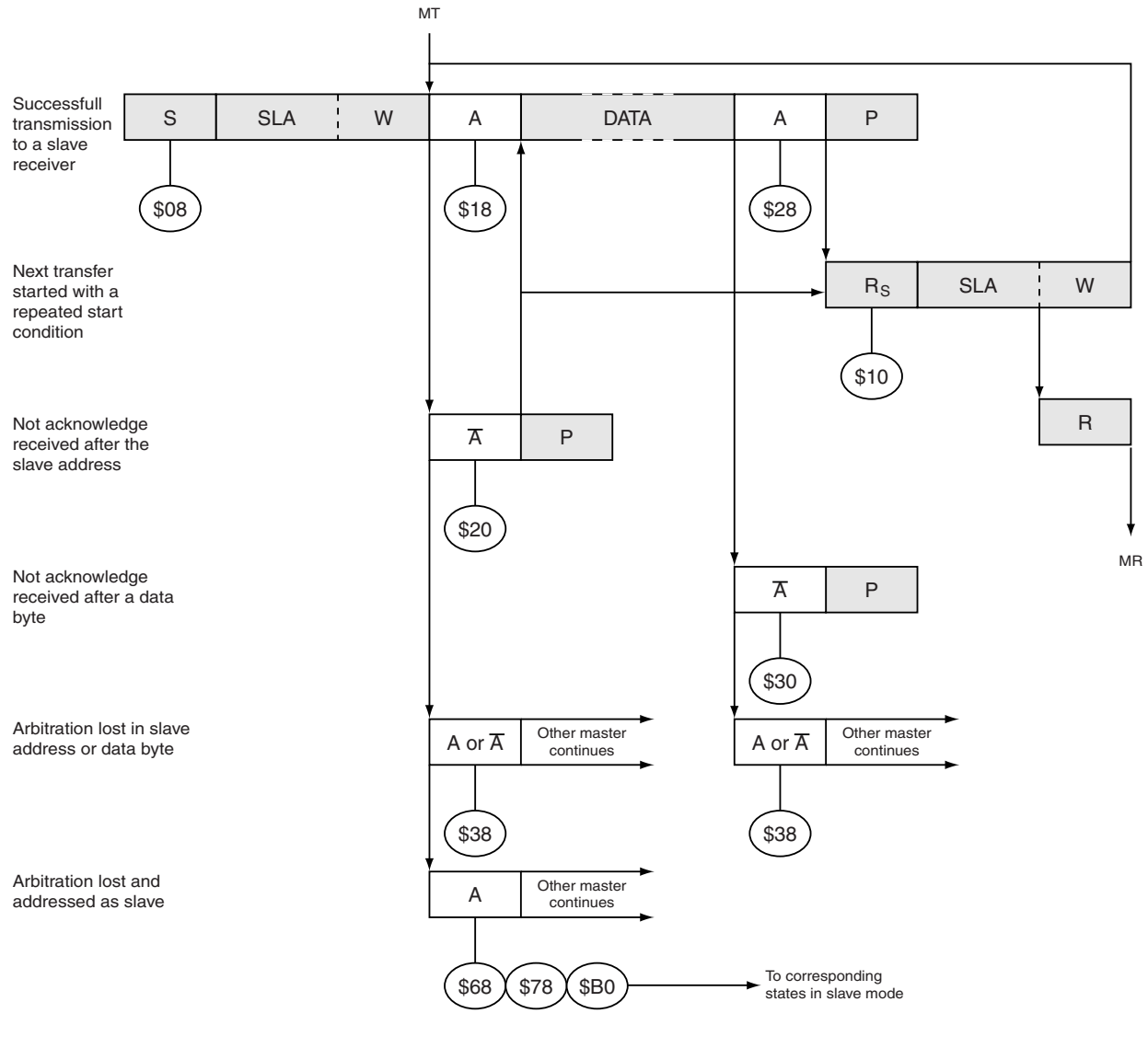
Figure 101. Formats and States in the Master Transmitter Mode
