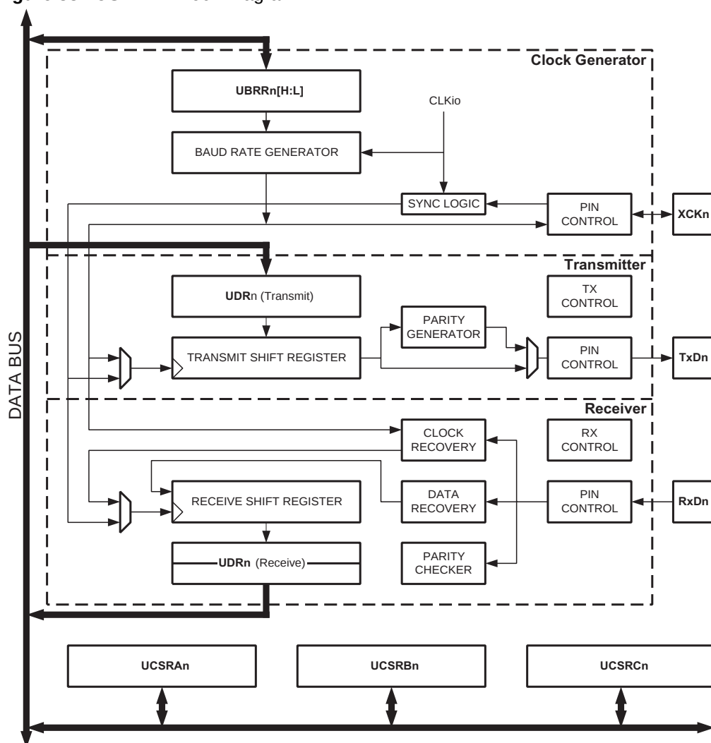
Figure 83. USARTn Block Diagram (1)
