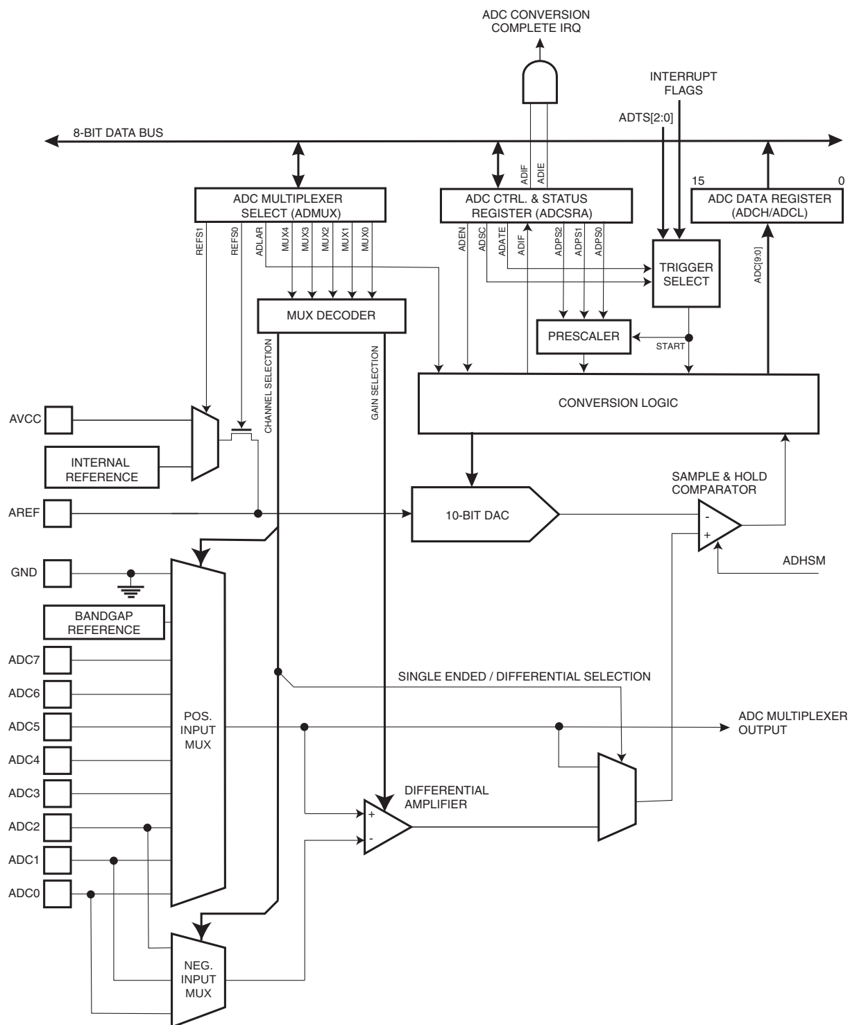
Figure 127. Analog to Digital Converter Block Schematic
