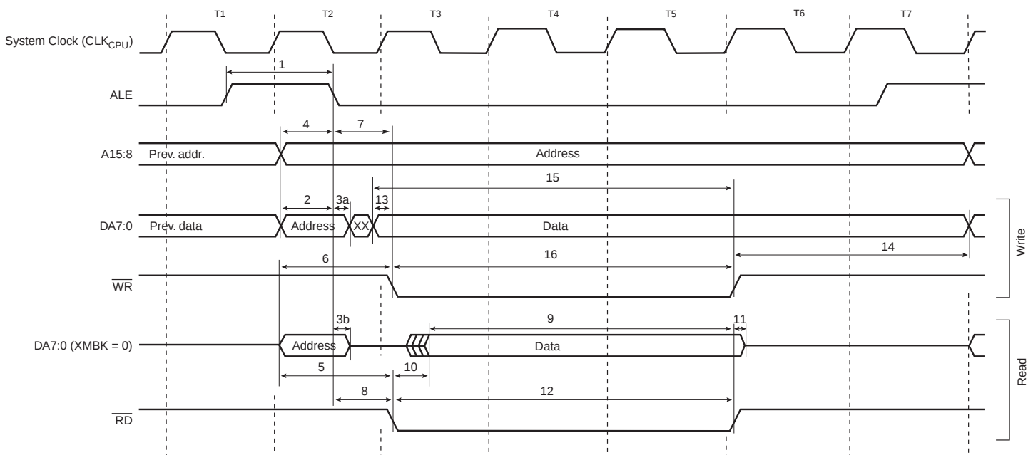
Figure 176. External Memory Timing (SRWn1 = 1, SRWn0 = 1) (1)
