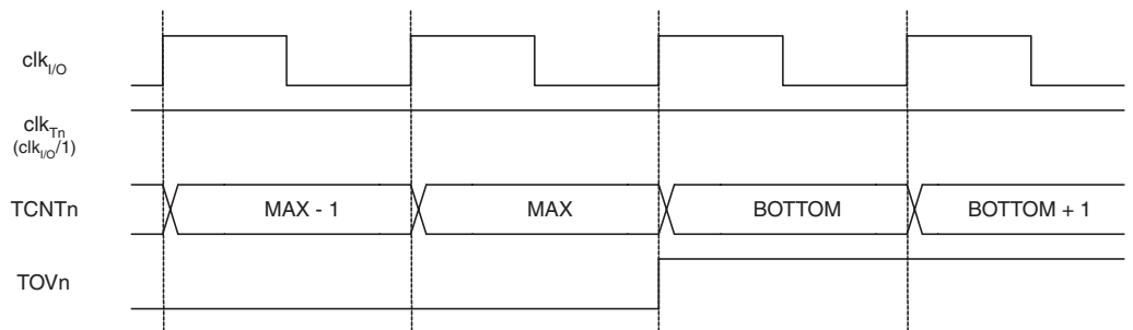
Figure 69. Timer/Counter Timing Diagram, no Prescaling
