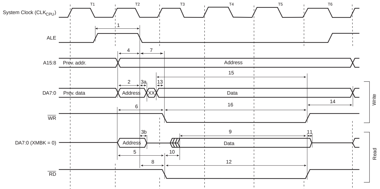
Figure 175. External Memory Timing (SRWn1 = 1, SRWn0 = 0)
