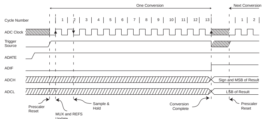
Figure 132. ADC Timing Diagram, Auto Triggered Conversion
