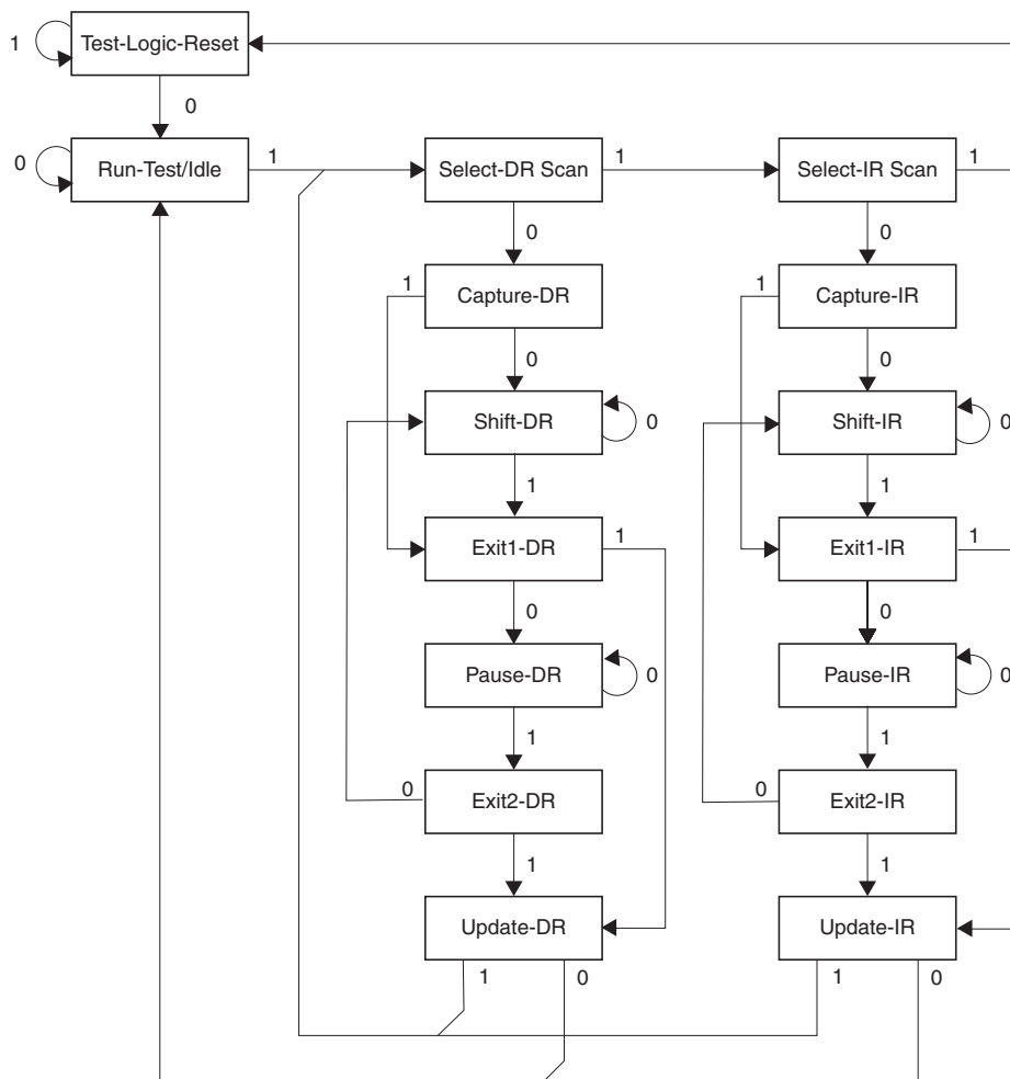
Figure 142. TAP Controller State Diagram
