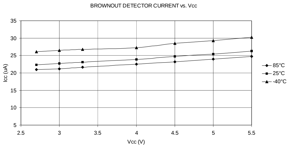
Figure 210. Brownout Detector Current vs. Operating Voltage
