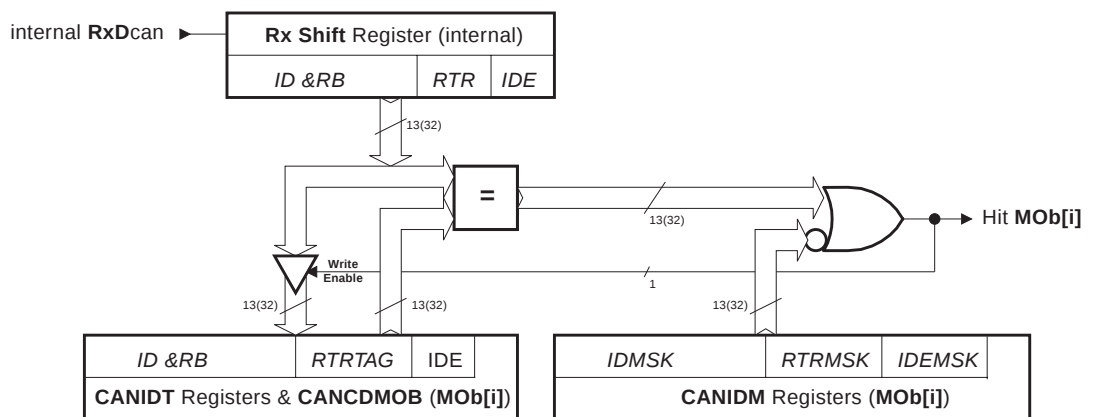
Figure 120. Acceptance Filter Block Diagram
