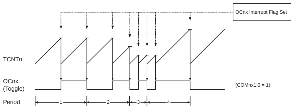
Figure 66. CTC Mode, Timing Diagram
