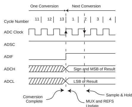
Figure 133. ADC Timing Diagram, Free Running Conversion
