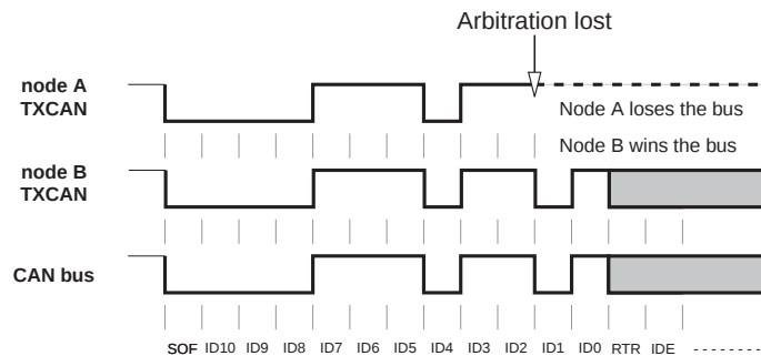
Figure 114. Bus Arbitration
