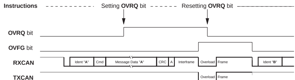
Figure 119. Overflow Frame
