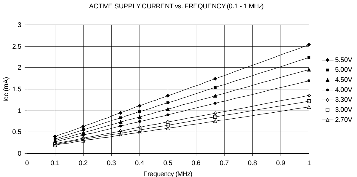
Figure 180. Active Supply Current vs. Frequency (0.1 - 1.0 MHz)
