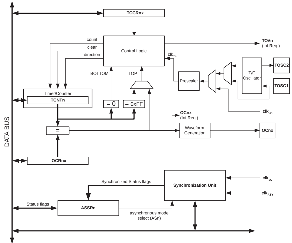
Figure 61. 8-bit Timer/Counter2 Block Diagram
