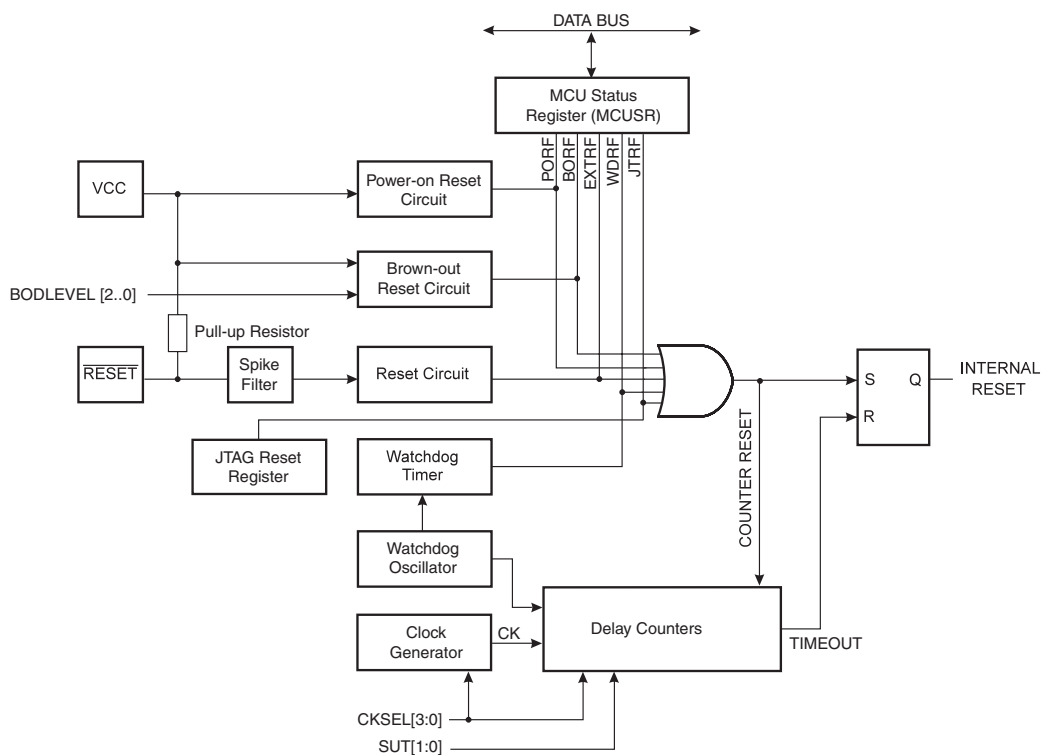
Figure 23. Reset Logic
