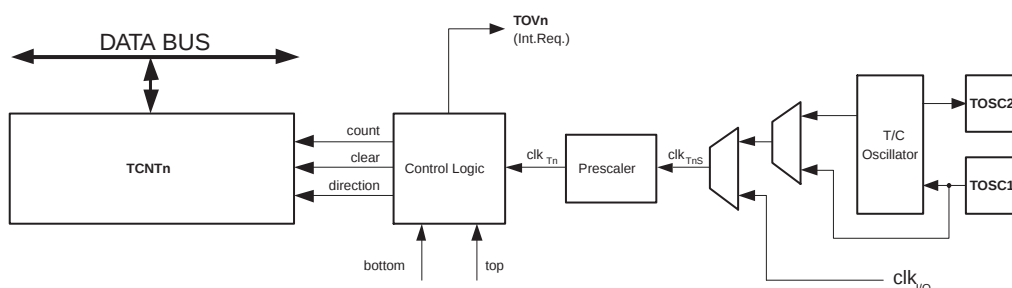
Figure 62. Counter Unit Block Diagram
