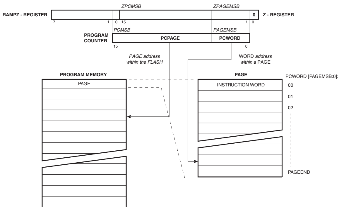
Figure 155. Addressing the Flash During SPM (1)
