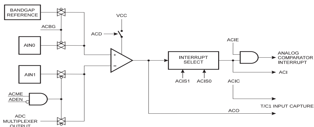
Figure 126. Analog Comparator Block Diagram (1)(2)
