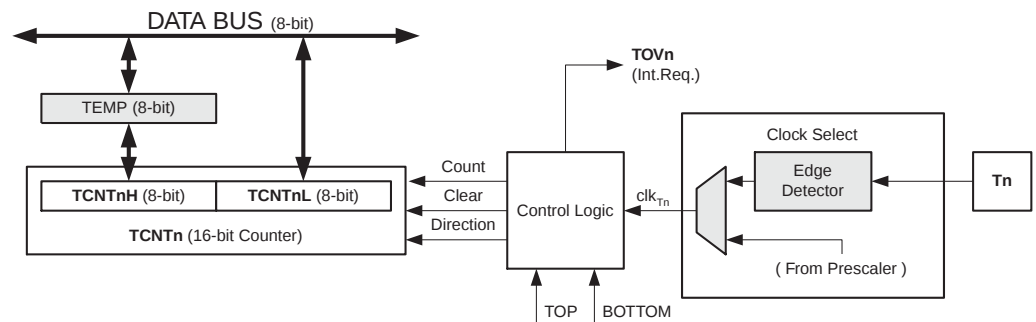
Figure 49. Counter Unit Block Diagram
