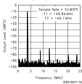
Two Tone Output Spectrum
