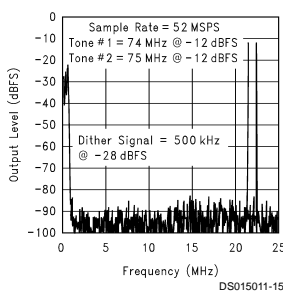
Two Tone Output Spectrum (with Dither)
