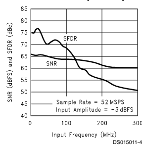
SNR and SFDR vs Input Frequency
