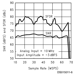
SNR and SFDR vs Sample Rate
