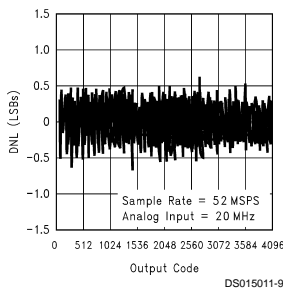
Differential Non-Linearity
