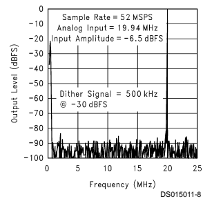
Single Tone Output Spectrum (with Dither)
