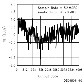
Integral Non-Linearity
