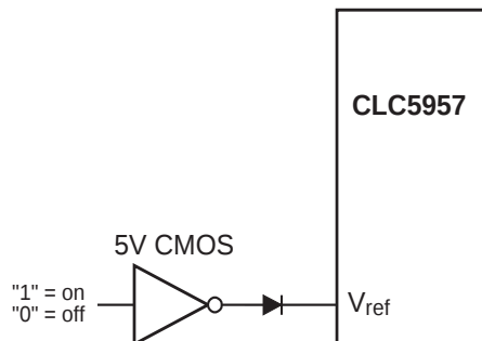
Figure 2: Power Shutdown Scheme
