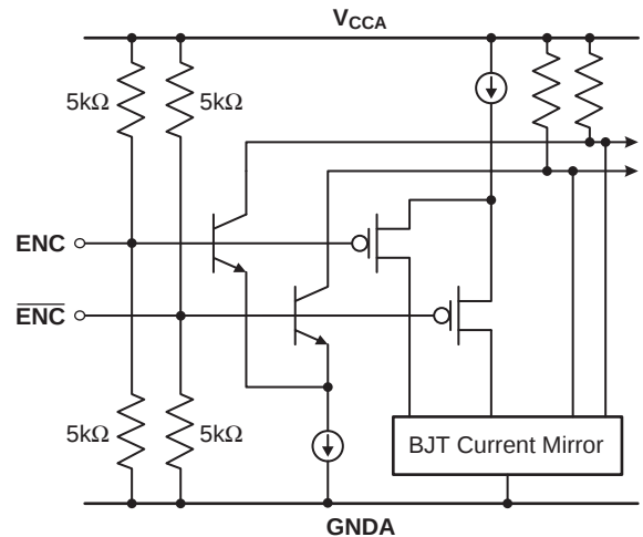
Figure 3: CLC5957 ENCODE Clock Inputs
