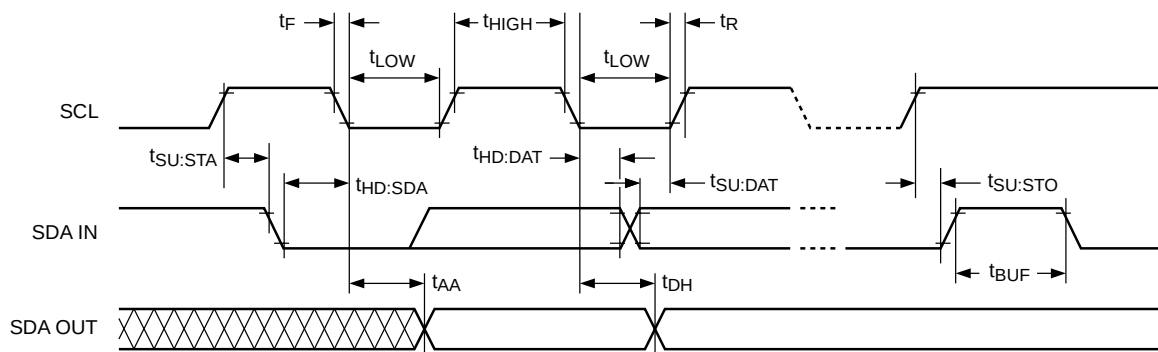
Figure 4. Bus Timing
