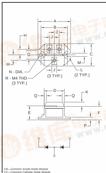
Outline Drawing
