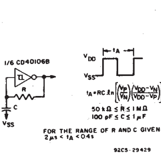
Fig. 18 - Astable multivibrator.
