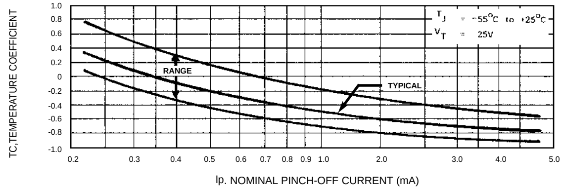
FIGURE 3 TEMPERATURE COEFFICIENT
