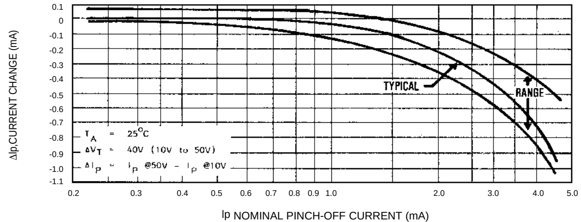
FIGURE 4 TEMPERATURE COEFFICIENT
