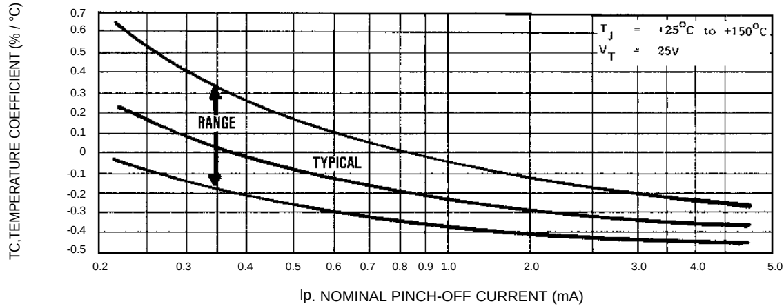
FIGURE 2 TEMPERATURE COEFFICIENT
