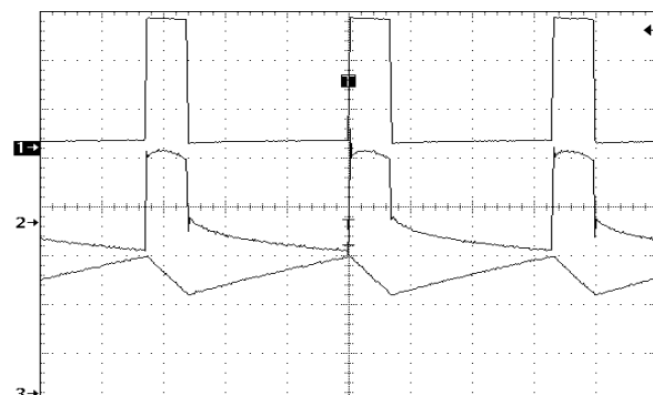
Figure 42. NCP1402SN30T1 Operating Waveforms (Heavy Load)
