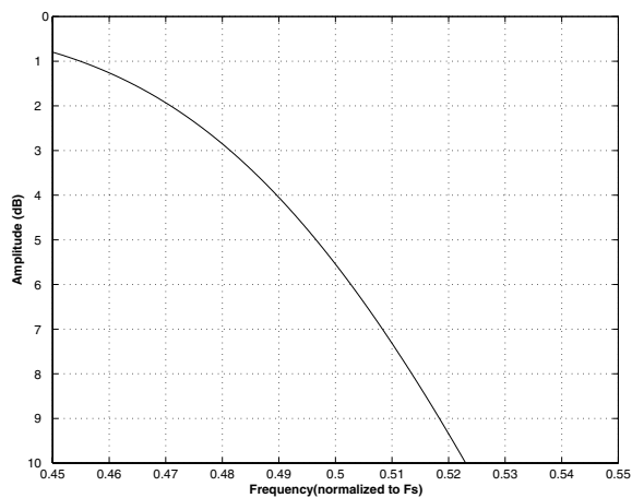
Figure 54. Quad Speed (slow) Transition Band (detail)
