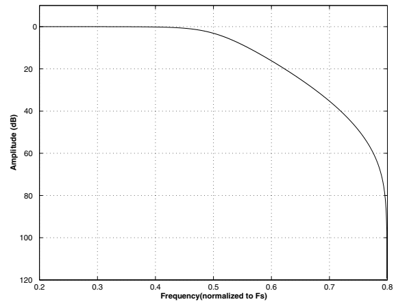
Figure 45. Double Speed (slow) Transition Band
