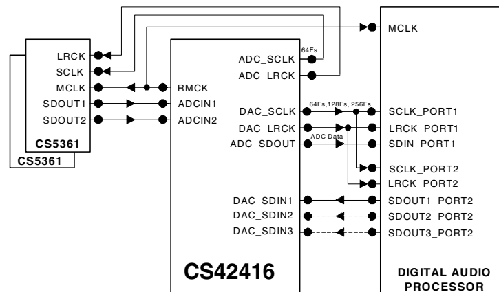
Figure 13. OLM Configuration #1
