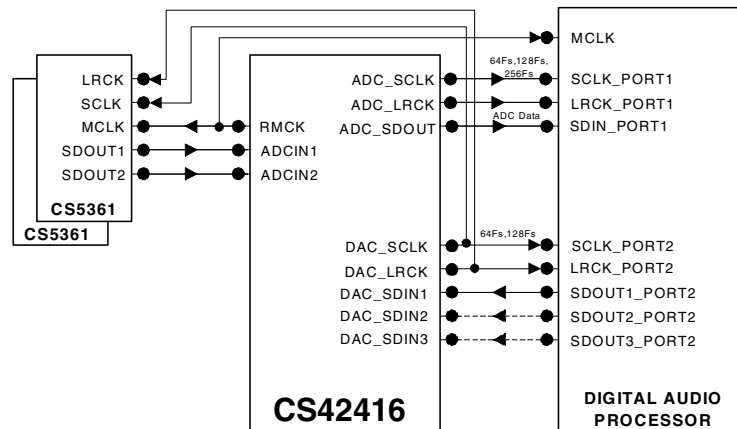
Figure 14. OLM Configuration #2
