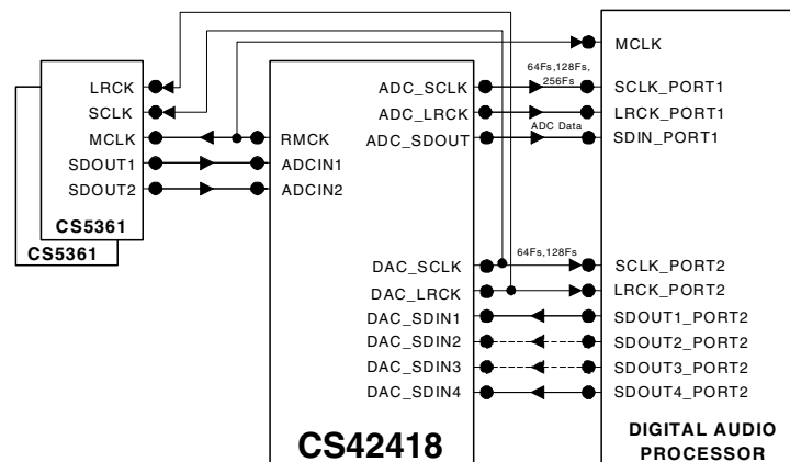
Figure 14. OLM Configuration #2
