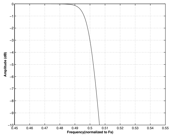
Figure 15. Single Speed (fast) Transition Band (detail)
