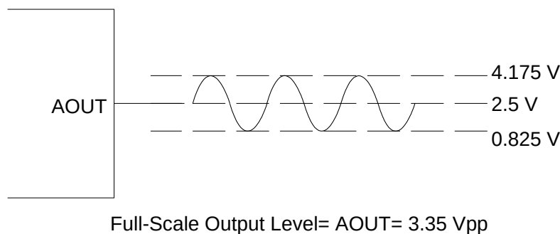
Figure 21. Full-Scale Output
