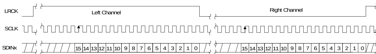
Figure 11. Format 2 - Right-Justified 16-bit Data
