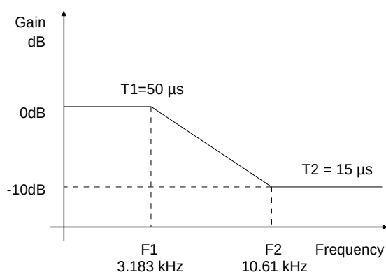
Figure 18. De-Emphasis Curve
