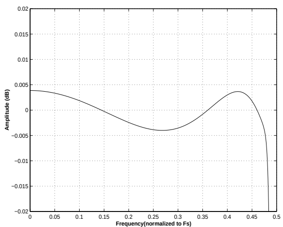
Figure 29. Single-Speed (fast) Passband Ripple
