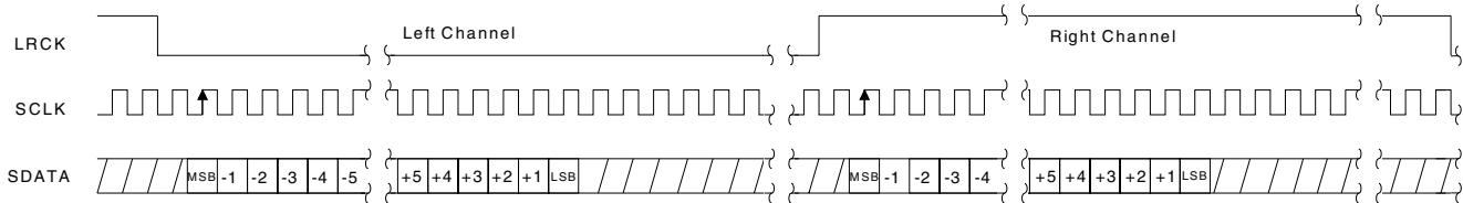
Figure 2. I²S Data
