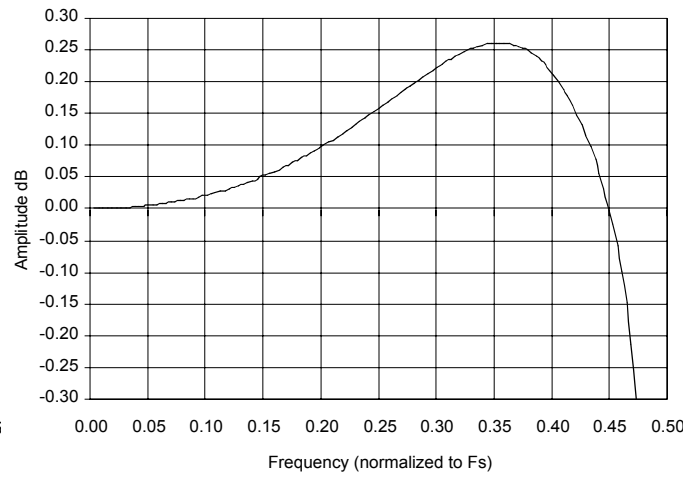
Figure 18. Double-Speed Passband Ripple
