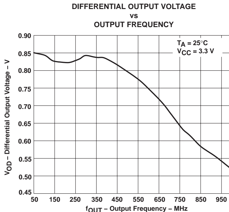
Figure 6. Differential Output Swing ( V_{OD} ) vs Frequency
