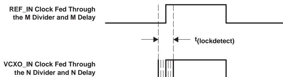
Figure 3. State Machine Operation
