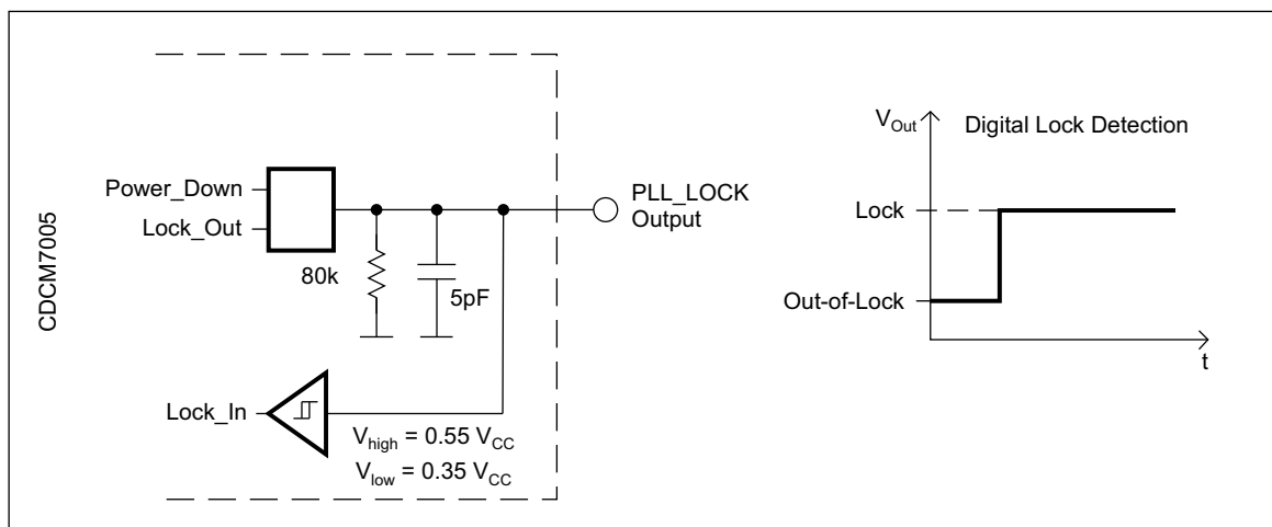
Figure 18. Digital Lock-Detect
