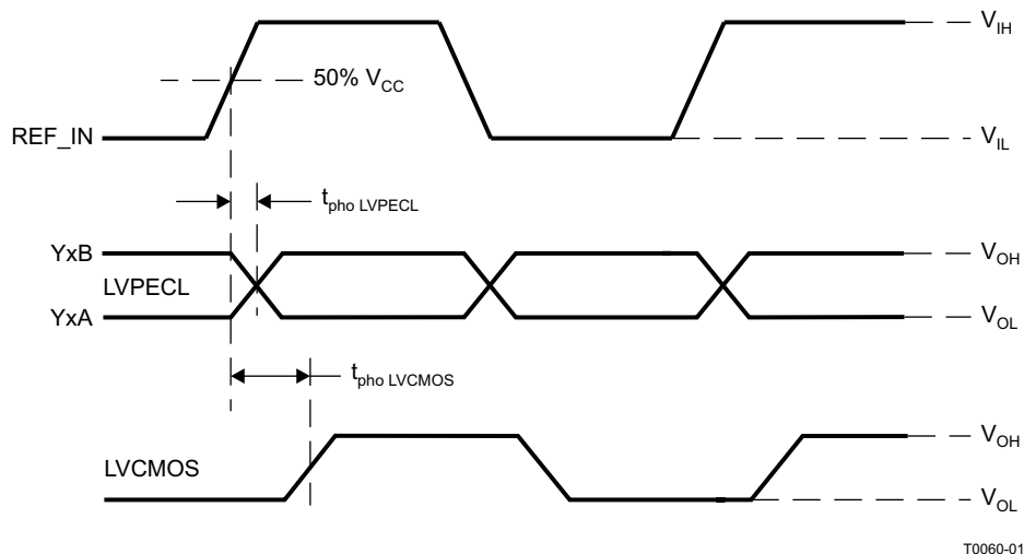
Figure 11. Phase Offset
