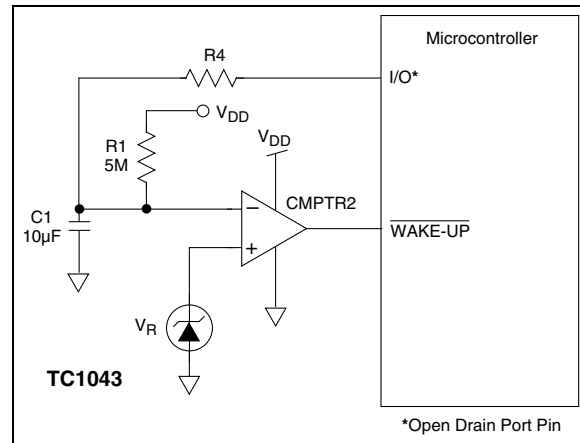
FIGURE 4-1: WAKE-UP TIMER
