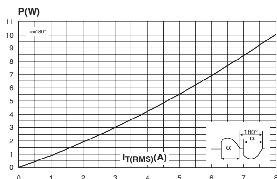
Figure 4: Maximum power dissipation versus RMS on-state current
