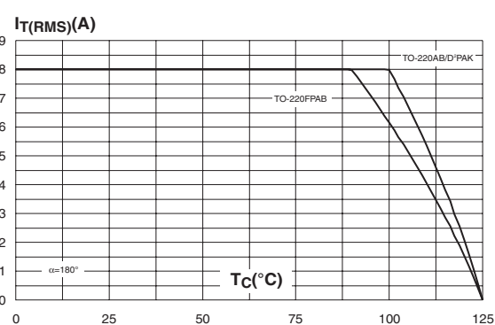
Figure 5: RMS on-state current versus case temperature
