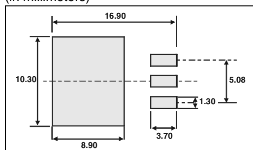
Figure 21: Foot Print Dimensions (in millimeters)
