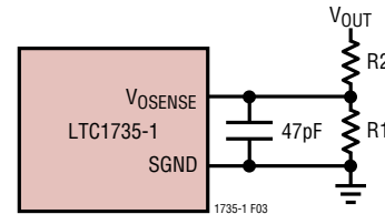
Figure 3. Setting the LTC1735-1 Output Voltage
