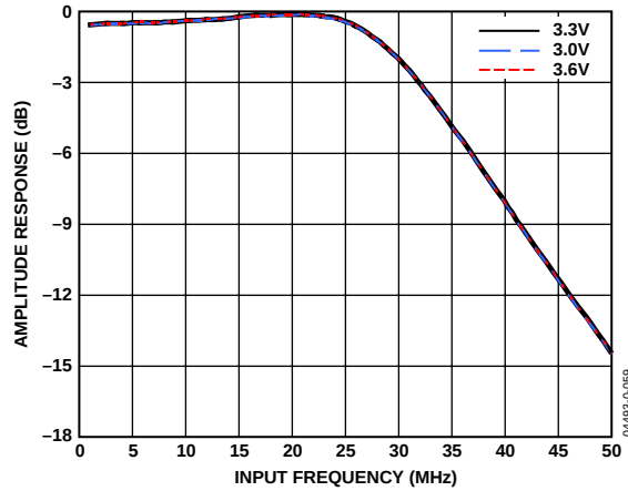
Figure 22. Rx Low-Pass Filter Amplitude Response vs. Supply ( f_{ADC} = 50\text{ MSPS} , f_{-3\text{ dB}} = 33\text{ MHz} , RxPGA = 0 dB)
