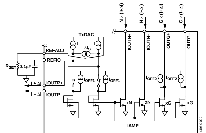
Figure 62. Equivalent Schematic of TxDAC and IAMP
