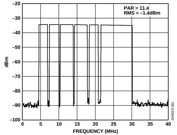
Figure 36. Spectral Plot of 111-Carrier OFDM Test Vector ( f_{\text{DATA}} = 80 \text{ MSPS} , 2\times Interpolation)
