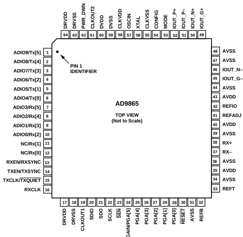
Figure 2. Pin Configuration
