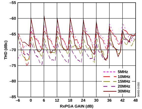
Figure 13. THD vs. R_{\text{xPGA}} Gain and Frequency
