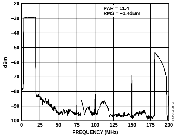
Figure 34. Wideband Spectral Plot of 88-Subcarrier OFDM Test Vector ( f_{\text{DATA}} = 50 \text{ MSPS} , 4\times Interpolation)
