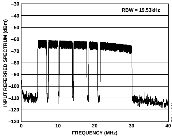
Figure 10. Spectral Plot with 4k FFT of 111-Carrier DMT Signal with \text{PAR} = 11 dB, P_{\text{IN}} = -33.7 dBm, LPF f_{-3\text{dB}} = 32 MHz, and R_{\text{xPGA}} = 36 dB
