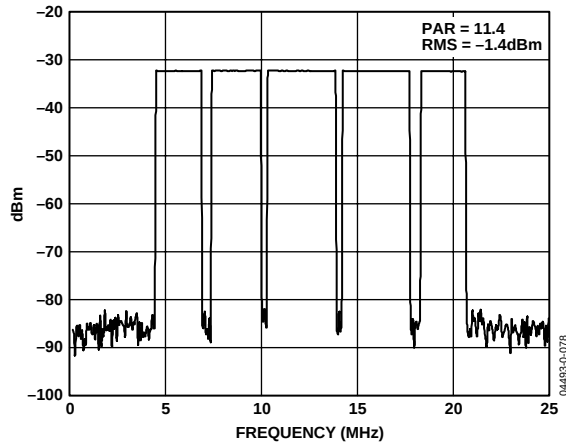
Figure 33. Spectral Plot of 84-Carrier OFDM Test Vector ( f_{\text{DATA}} = 50 \text{ MSPS} , 4\times Interpolation)
