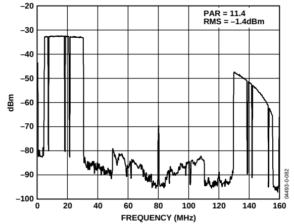
Figure 37. Wideband Spectral Plot of 111-Carrier OFDM Test Vector ( f_{\text{DATA}} = 80 \text{ MSPS} , 2\times Interpolation)
