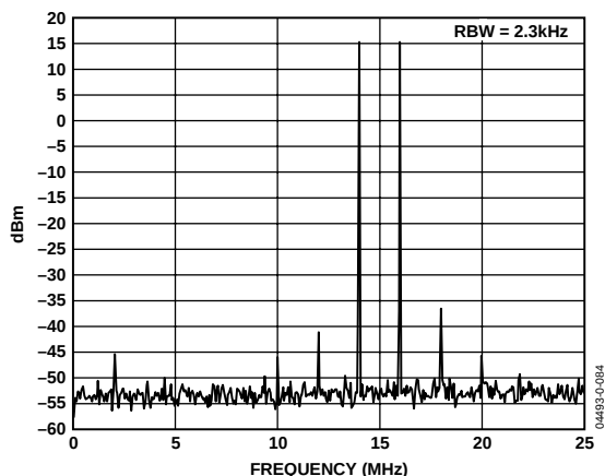
Figure 39. Dual-Tone Spectral Plot of IAMPN Output (IAMP Settings of I = 12.5 mA, N = 4 , G = 0 , 2:1 Transformer into 75 \Omega Loader, V_{\text{CM}} = 4.8 V)
