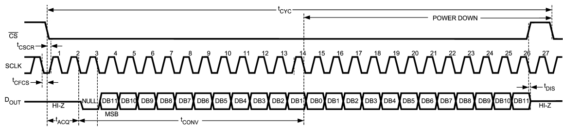
ADC121S625 Double Cycle Timing Diagram
