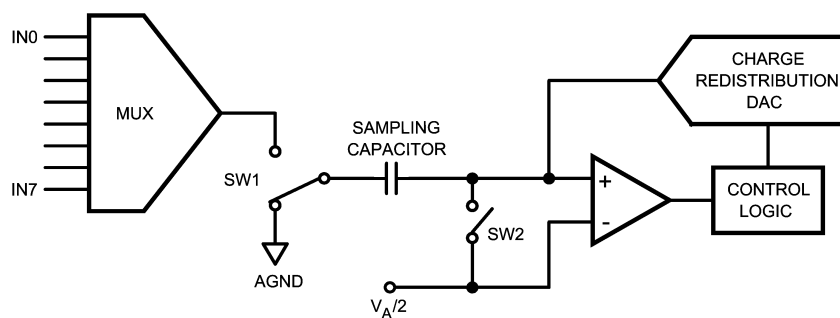
FIGURE 5. ADC128S022 in Hold Mode
