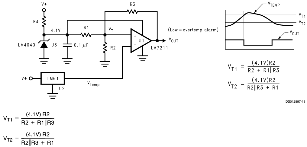
FIGURE 7. Centigrade Thermostat
