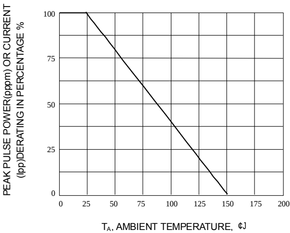
Fig. 2-PULSE DERATING CURVE
