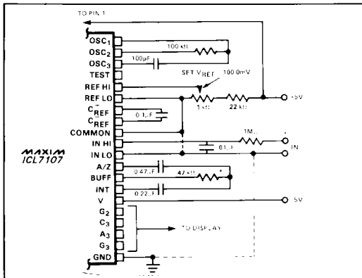
Figure 14. ICL7107 Internal Reference. 200mV Full Scale; 3 Readings per Second, V_{IN} Tied to GND for Single Ended Inputs. (See discussion under "Analog Common".)
