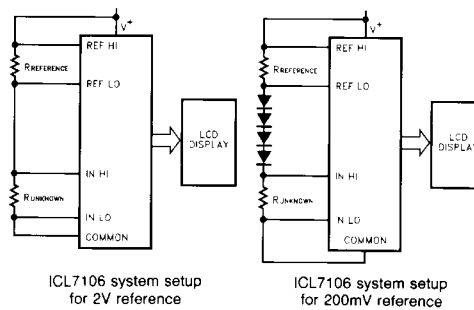
Figure 22. Ratimetric Ohms Measurement
