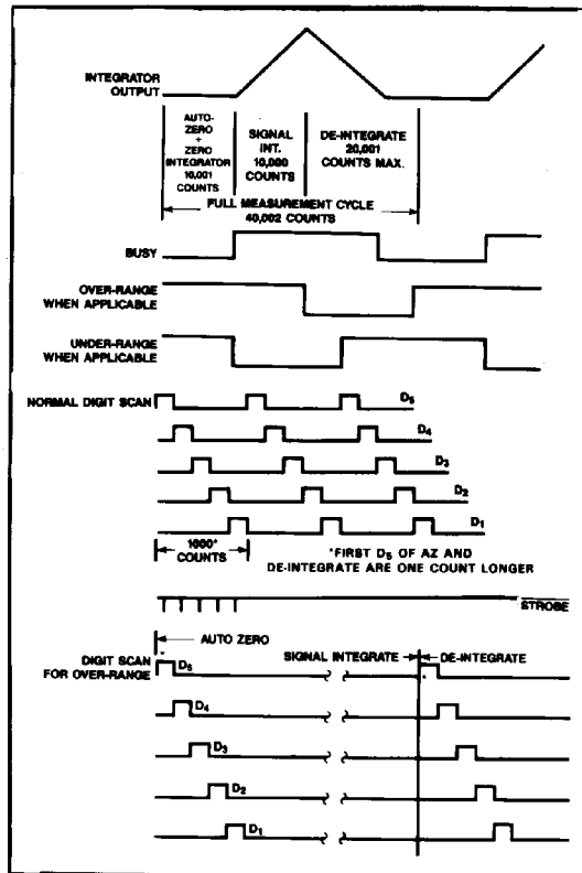
Figure 4. Timing Diagram
