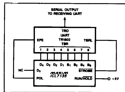
Figure 14. ICL7135 to UART Interface
